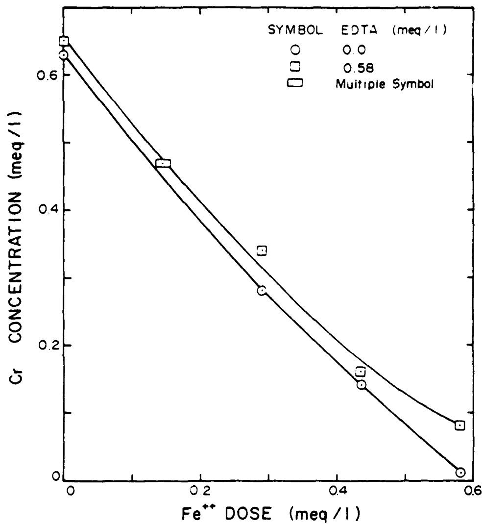
Figure 23. Effects of EDTA on chromium reduction by ferrous sulfate in hard tap water at pH 8.5.
