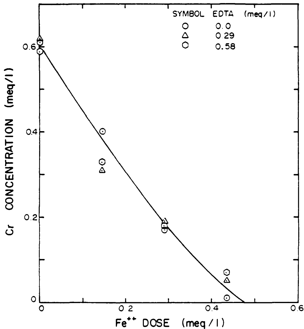
Figure 24. Effects of EDTA on chromium reduction by ferrous sulfate and sodium sulfide (0.29 meq/l) in hard tap water at pH 8.5.
