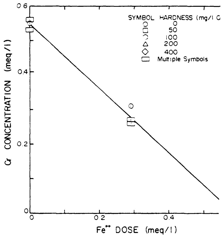
Figure 17. Effects of hardness and alkalinity (200 mg/l as \text{CaCO}_3 ) on chromium reduction by ferrous sulfate at pH 8.5.
