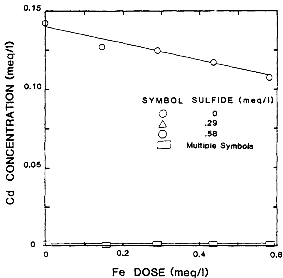
Figure 54. Cadmium (0.18 meq/l) removal from a mixed metal plating waste in hard tap water with pH adjusted to 8.5 with lime.
