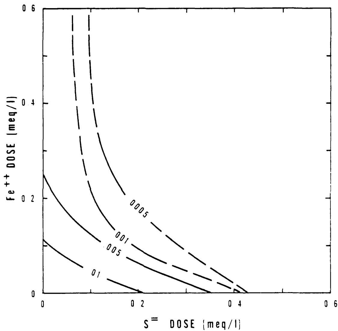
Figure 34. Isoequivalent cadmium residuals for treatment of mixed metals in softened tap water at pH 8.5.
