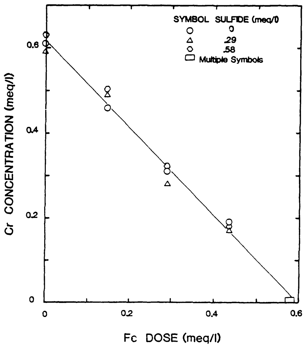
Figure 42. Chromium (0.58 meq/l) removal from a mixed metal waste in hard tap water ( \text{Ca}(\text{OH})_2 ) with pH adjusted to 8.5 with lime.
