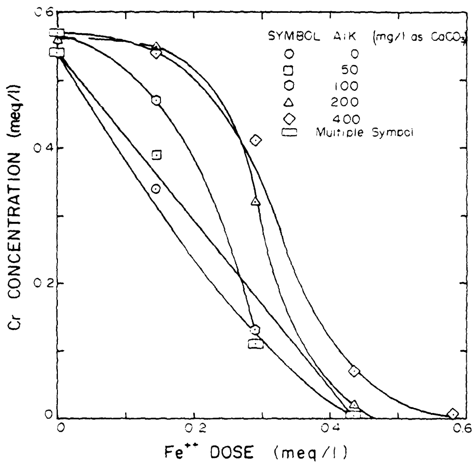
Figure 14. Effects of alkalinity on chromium reduction by ferrous sulfate and sodium sulfide (0.29 meq/l) at pH 3.5.
