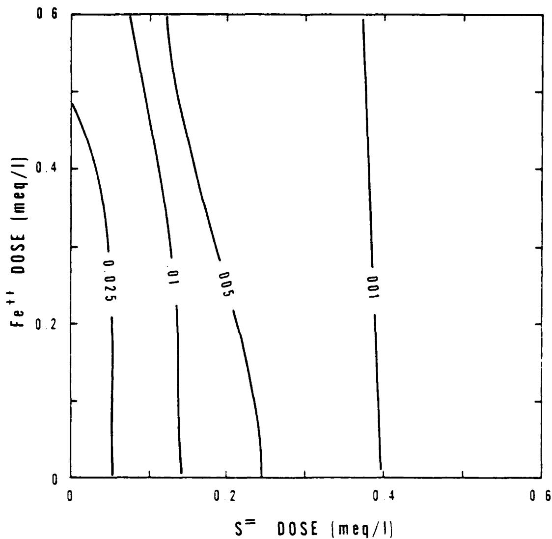
Figure 33. Isoequivalent cadmium residuals (meq/l) for treatment of mixed metals in softened tap water at pH 7.
