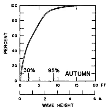
Figure 34 Seasonal wave height
