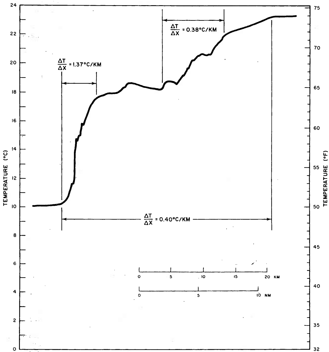
Figure 21 Multiple surface gradient, northern edge
