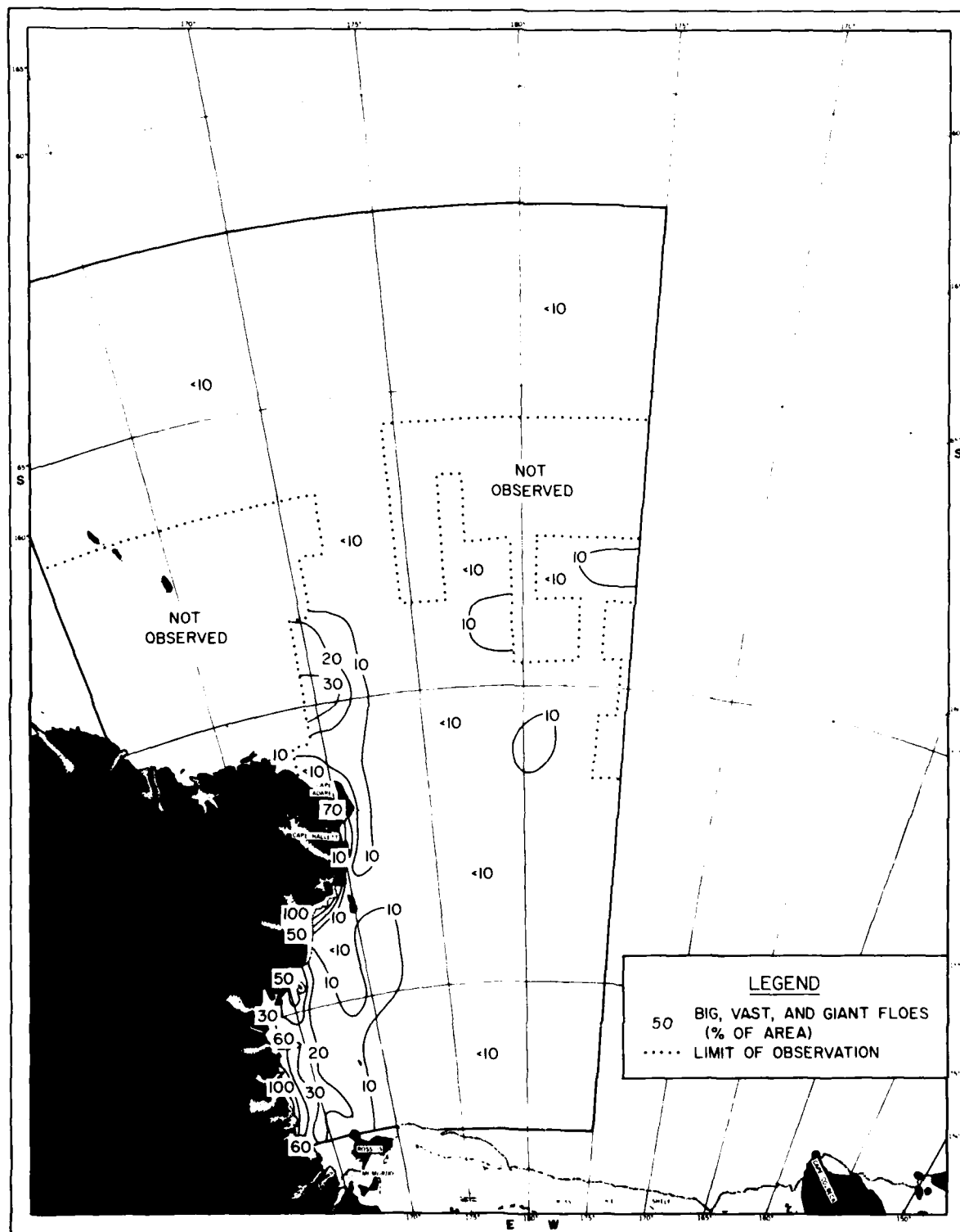
FIGURE C-12. FLOE SIZE 16-31 DECEMBER
