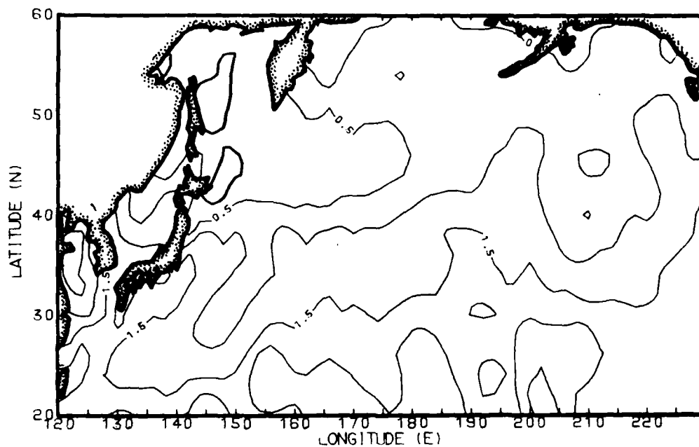
FIGURE 7.11 Monthly mean latent heat flux (ocean to atmosphere) is the mean of 12-hourly latent heat flux calculated from FNWC sea temperature, vapor pressure and wind using a bulk formula. Isoline of zero heat flux are plotted heavily, and contour intervals are 0.5 \times 10^{-3} cal/cm 2 sec.
