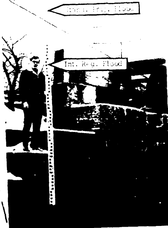
FIGURE 9 - Def. Rt. 7 at the Penn Central Railroad overpass. The Standard Project Flood would be 1.9 feet above top of rod.
