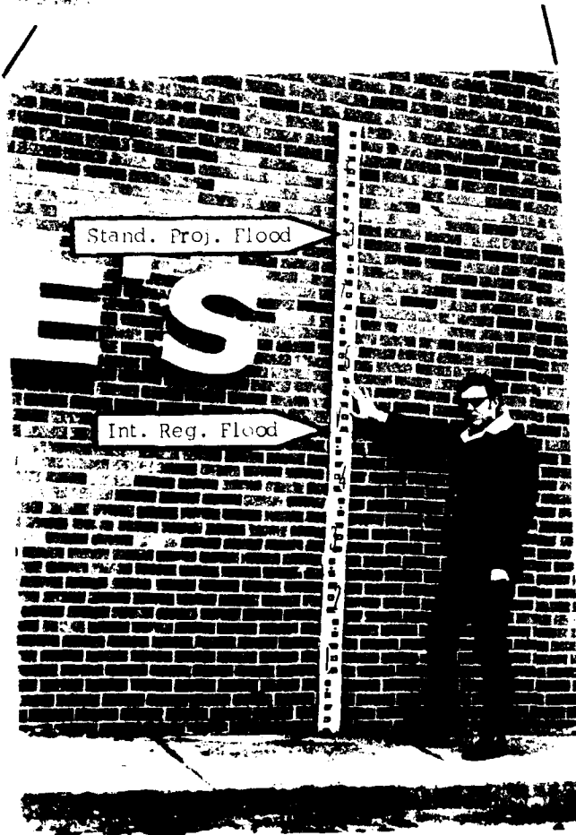
FIGURE 8 - Future flood heights at Lowe's of Wilmington located on Wilmington-Christina Pike (Del. Rt. 7)
