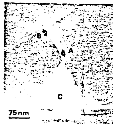
Fig. 4. Dark-field transmission electron micrograph revealing the presence of a continuous glass phase at the \text{Si}_3\text{N}_4/\text{Si}_3\text{Sc}_2\text{O}_7 grain junctions, A, and surrounding the \text{Sc}_2\text{Si}_2\text{O}_7 grain, B. Less apparent but also observable is the glass phase around the \text{Sc}_2\text{Si}_2\text{O}_7 grain, C.
