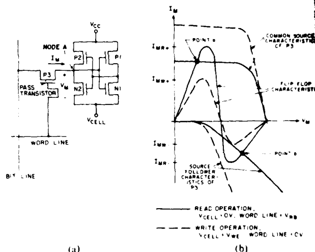
Fig. 1. (a) Five-transistor CMOS memory cell. (b) Current-voltage characteristics of flip-flop and word line transistor.
