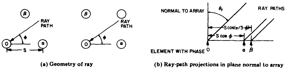
Fig. A6 — Geometry of rays for given array phase distribution
