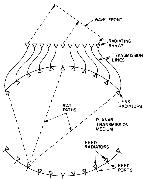
Fig. 1 — Gent/Rotman bootlace lens (2D)
