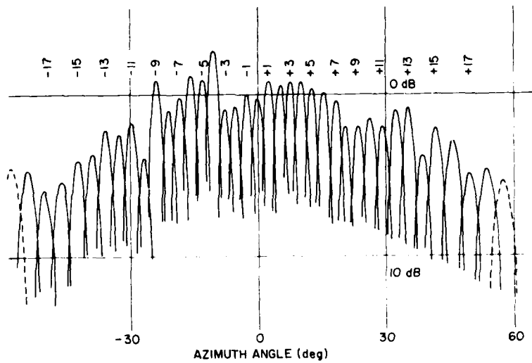
Fig. 10 — Combined plot of all beams from 37-element linear array
