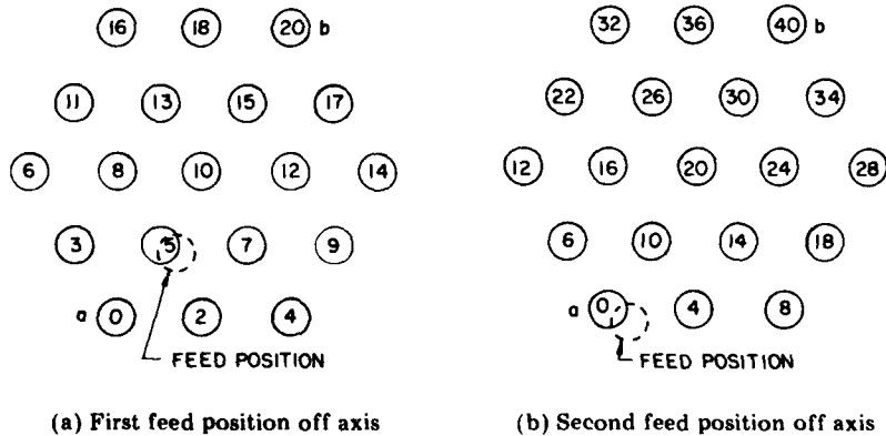
Fig. 5 - Integer aperture distributions for 19-element hexagonal array
