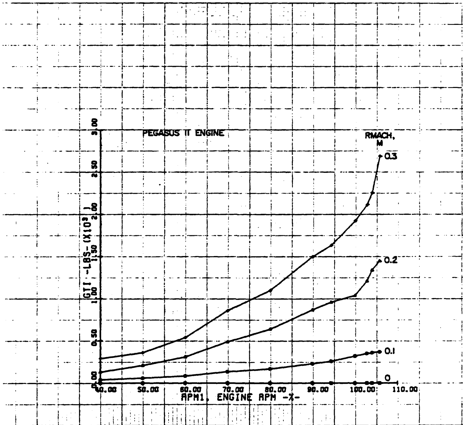
FIGURE 60 - Gross Thrust Increase Due to Freestream Velocity.
