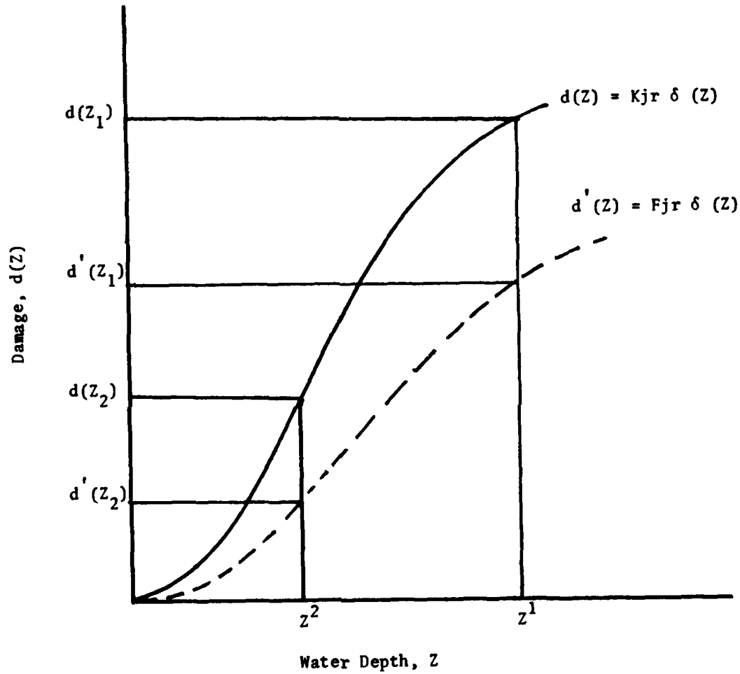
Figure III-4 Two Methods of Floodproofing 8
