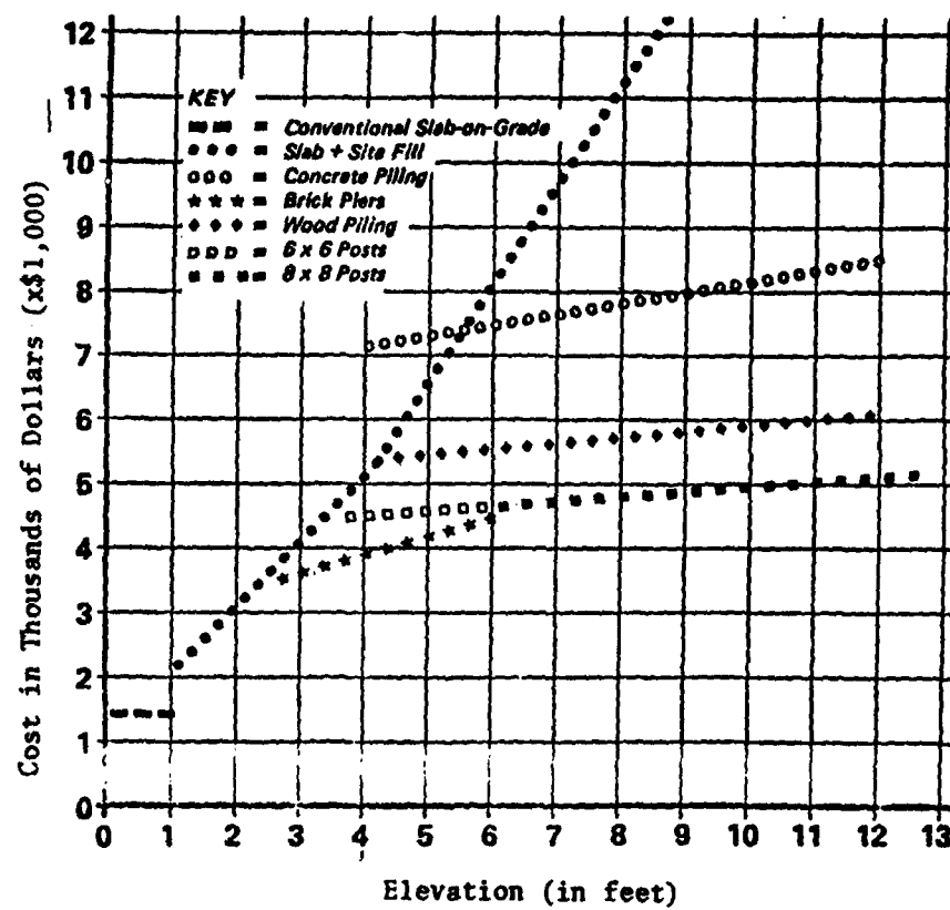
Figure A-5 Cost Comparison of Foundation Types for a Specific House in Louisiana
