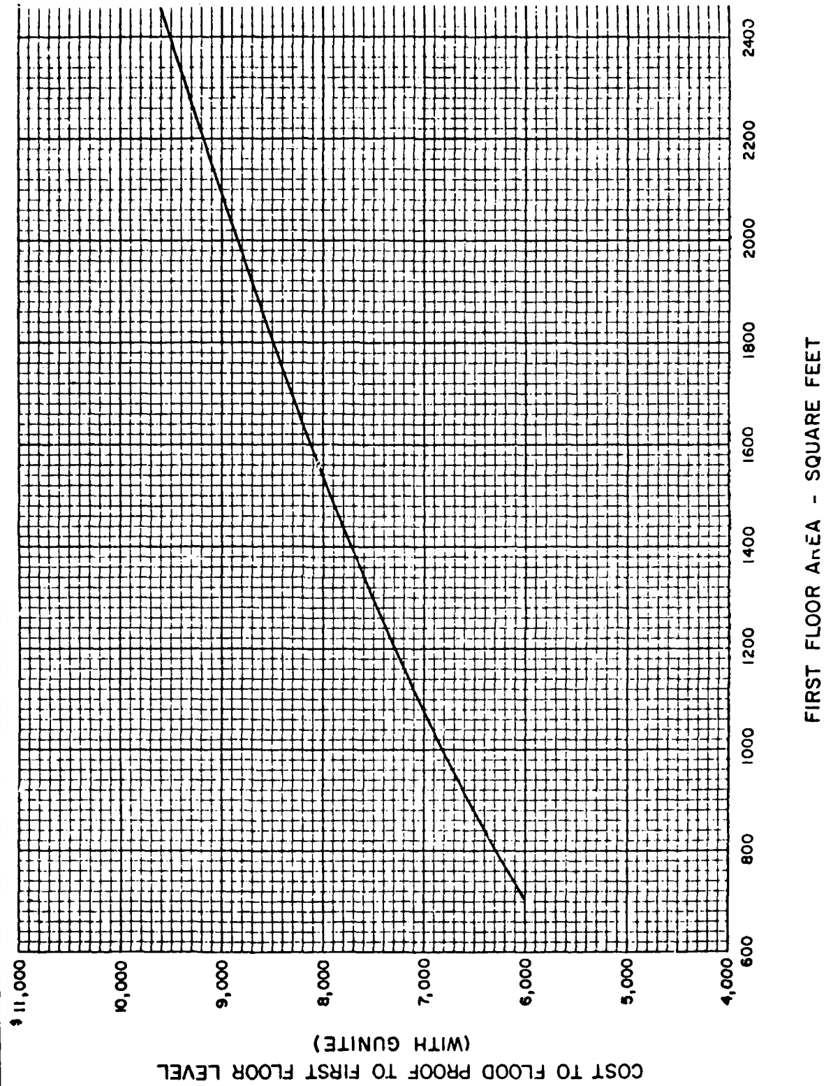
Figure A-1 Relation Between Floodproofing Costs and Size of Structure
