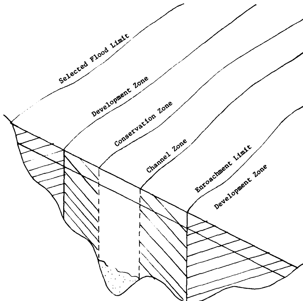
Figure II-3 Floodplain Utilization
