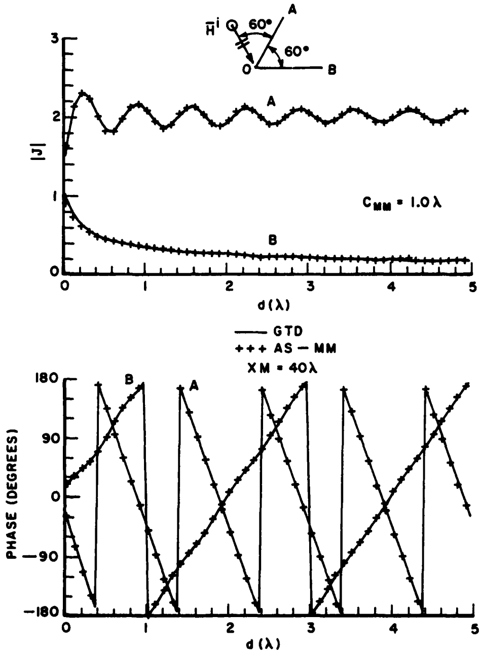
Figure 3.11. Currents on a wedge for \phi_w = 60^\circ , \phi = 60^\circ , C_{MM} = 1.0\lambda , and XM = 40\lambda .
