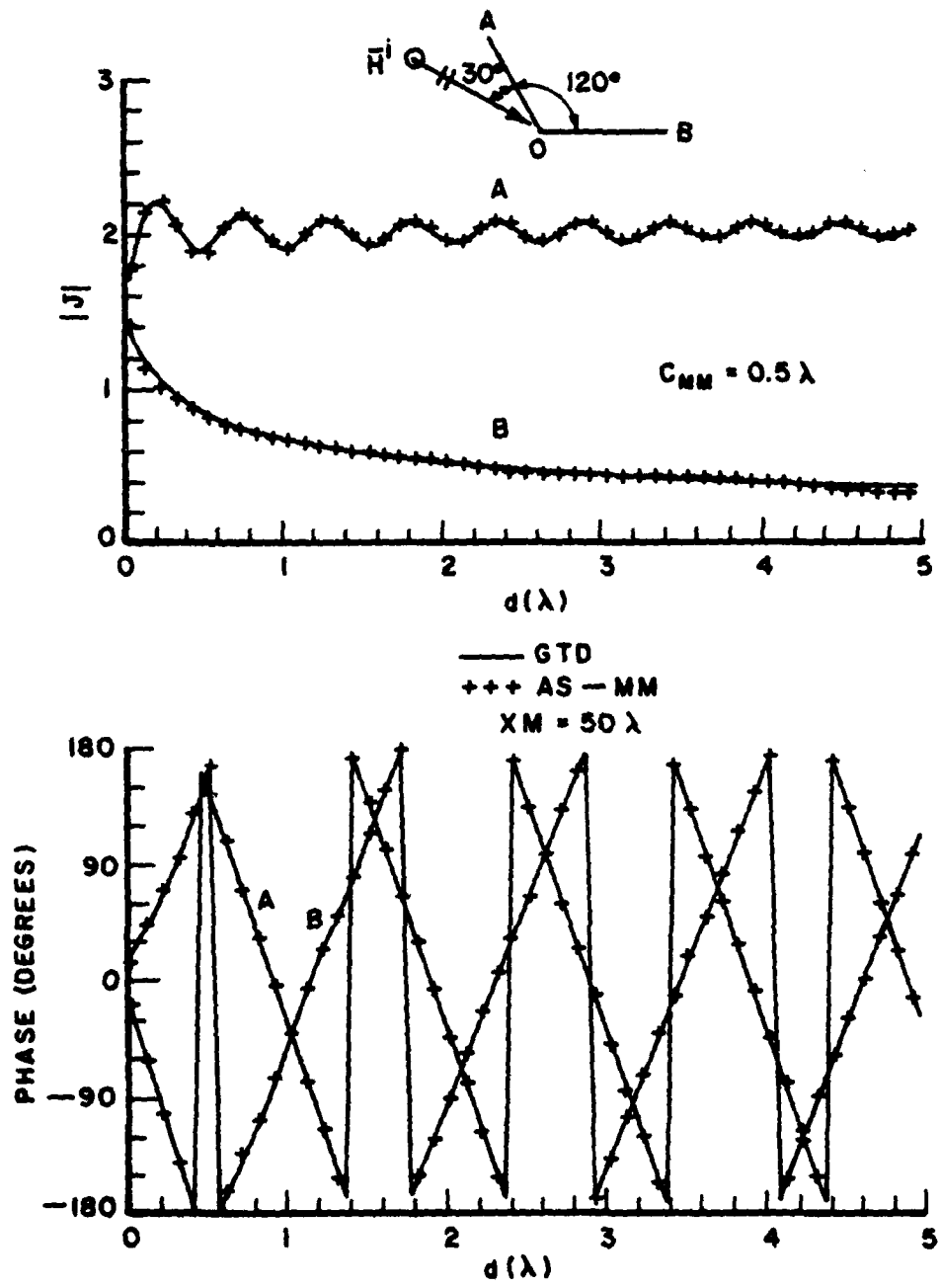
Figure 3.7. Currents on a wedge for \phi_w = 120^\circ , \phi_i = 30^\circ , C_{MM} = 0.5\lambda , and XM = 50\lambda .
