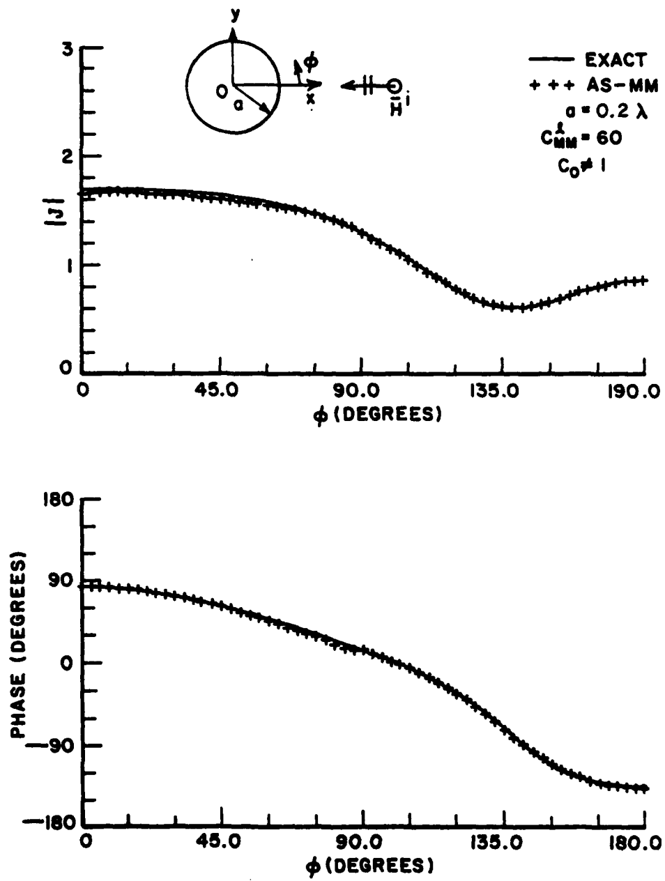
Figure 5.5. Current on a circular cylinder for a=0.2\lambda , C_{MM}^{\lambda}=60^{\circ} , and C_0 \neq 1 .
