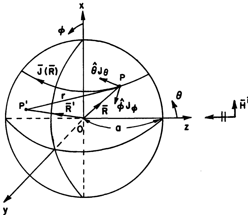
Figure 6.1 Geometry of a sphere illuminated by the x-polarized plane wave.
