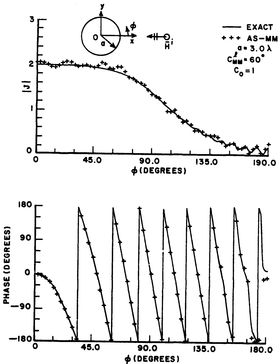
Figure 5.13. Current on a circular cylinder for a=3.0\lambda , C_{MM}^\lambda=60^\circ , and C_0=1 .
