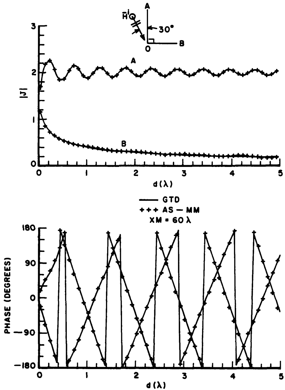
Figure 3.5. Currents on a wedge for \phi_w = 90^\circ , \phi_i = 30^\circ , C_{MM} = 0.5\lambda , and XM = 60\lambda .
