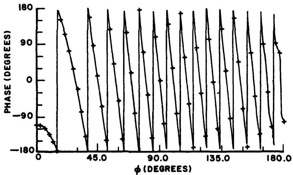
Figure 5.8. Current on a circular cylinder for a=5.7\lambda , C_{MM}^{\lambda}=60^{\circ} , and C_0 \neq 1 .
