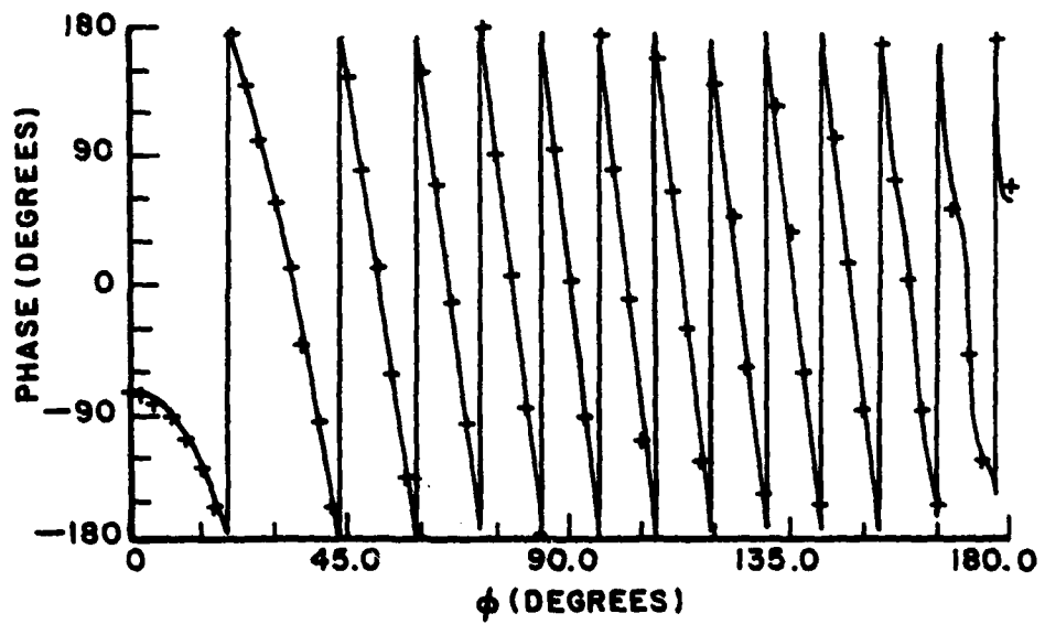
Figure 5.11. Current on a circular cylinder for a=4.8\lambda , C_{MM}^l=60^\circ , and C_0=1 .
