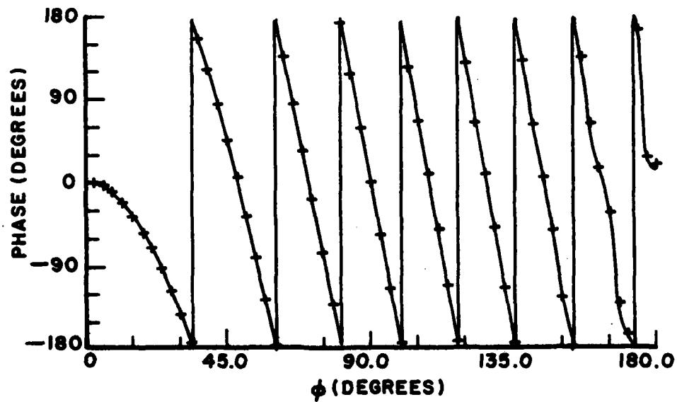
Figure 5.14. Current on a circular cylinder for a=3.0\lambda , C_{MM}^l=60^\circ , and C_0 \neq 1 .
