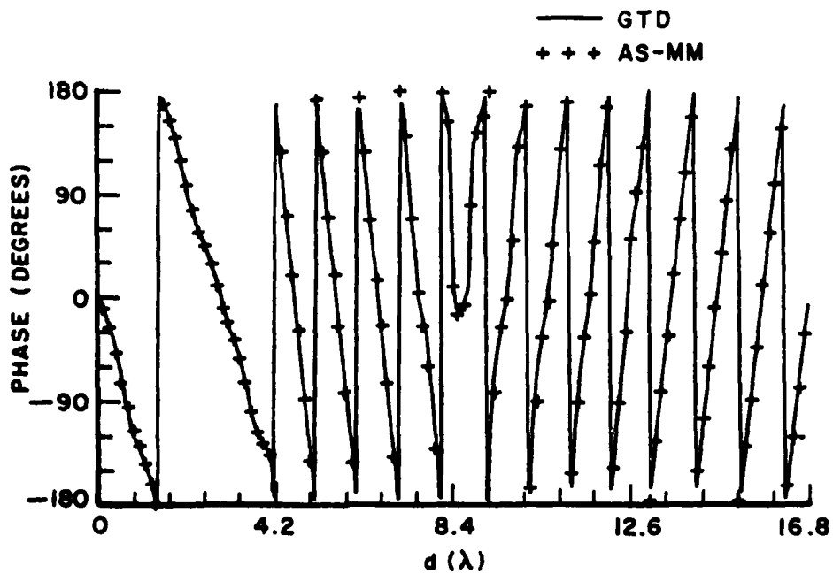
Figure 4.5. Current on a square cylinder for W=4.2\lambda , \theta_i=110^\circ , and C_{MM}=0.5W .
