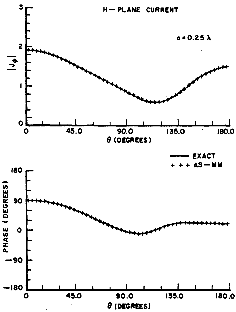
Figure 6.5. The H-plane current on a sphere for a=0.25\lambda , N=24 , and S_{MM}=30^\circ .
