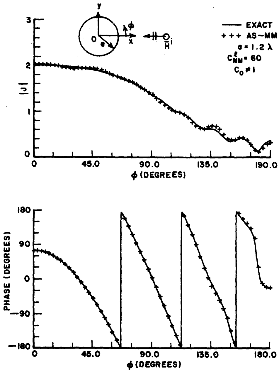
Figure 5.6. Current on a circular cylinder for a=1.2\lambda , C_{MM}^{\beta}=60^{\circ} , and C_0 \neq 1 .
