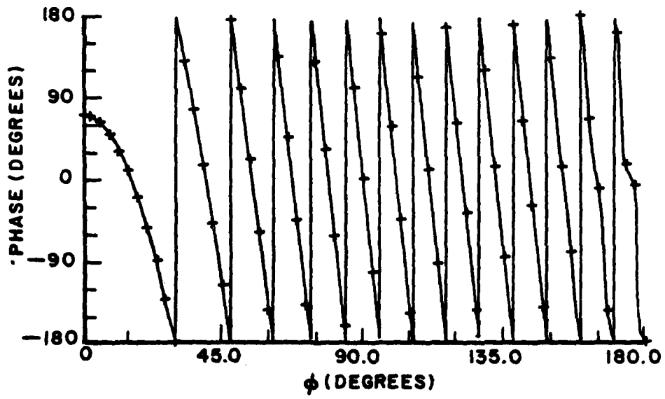
Figure 5.10. Current on a circular cylinder for a=5.2\lambda , C_{MM}^l=120^\circ , and C_0 \neq 1 .
