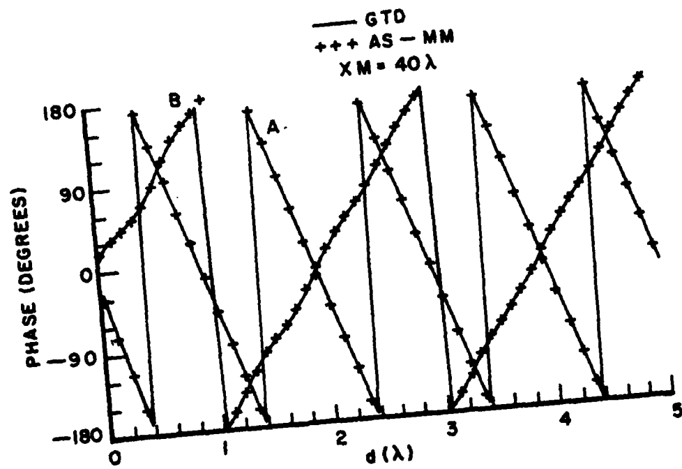
Figure 3.10. Currents on a wedge for \phi_w = 60^\circ , \phi_i = 60^\circ , C_{MM} = 0.25\lambda , and XM = 40\lambda .
