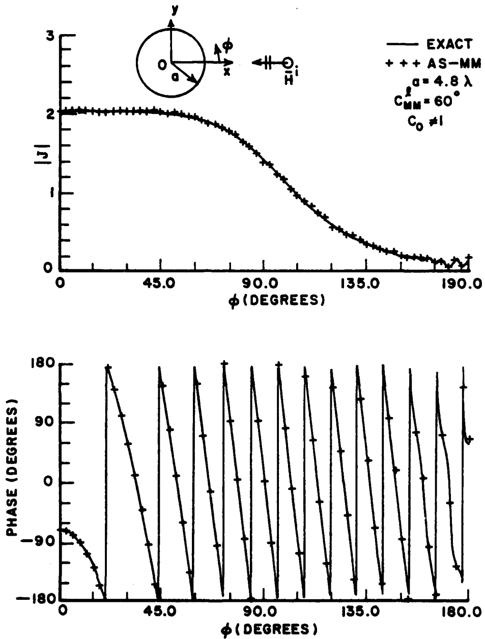
Figure 5.12. Current on a circular cylinder for a=4.8\lambda , C_{MM}^L=60^\circ , and C_0 \neq 1 .
