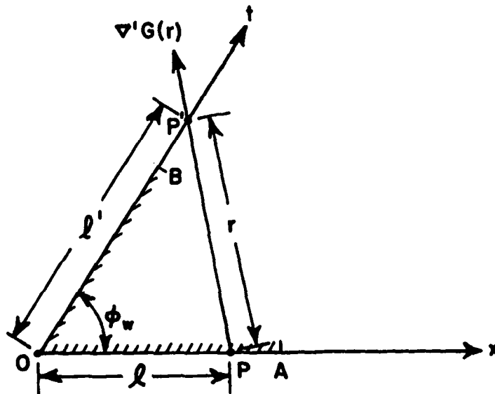
Figure 3.3. Geometry showing relationship between l , l' , and \phi_w in a wedge.
