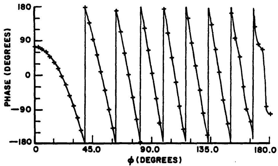
Figure 5.7. Current on a circular cylinder for a=3.2\lambda , C_{MM}^2=60^\circ , C_0 \neq 1 .
