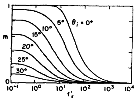
Figure 18. Envelope Variation vs. PRF \theta_d = 0^\circ , SNR=6 dB, INR=40 dB, \delta = .001
