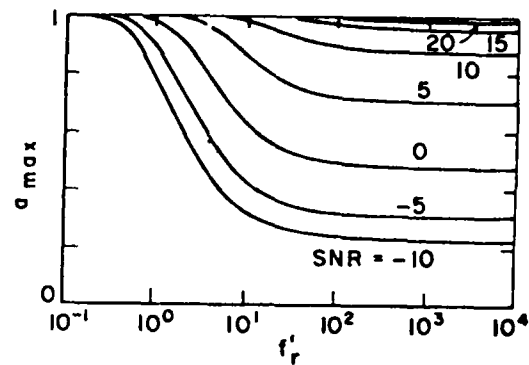
Figure 25. Envelope Peak vs. PRF \theta_d=0^\circ , \theta_i=10^\circ , INR=40 dB, \tau'=.0001
