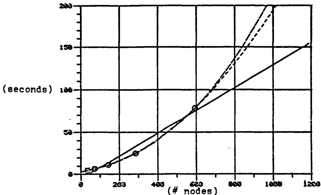
Figure 5 - CPU time vs problem size (PLATE)
