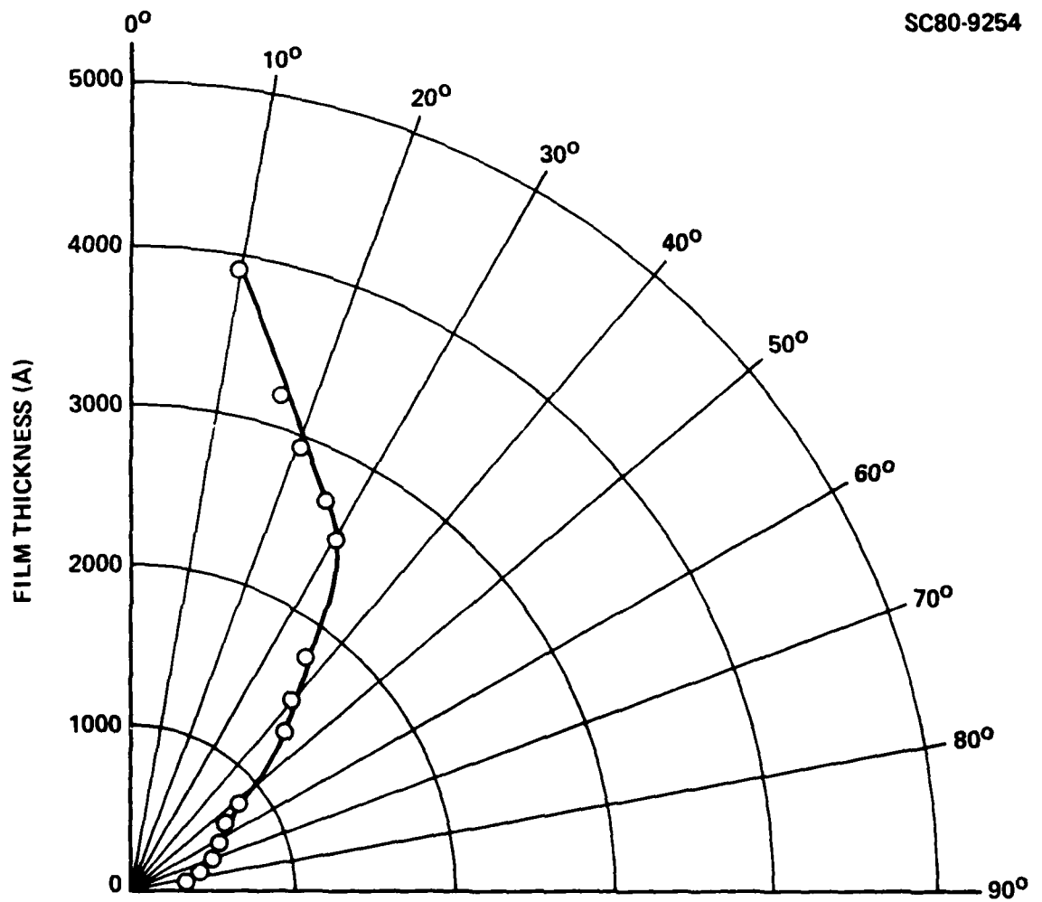
Fig. 8 Angular dependence of the film thicknesses.
