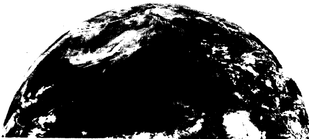
Figure 9a. GOES WEST INFRARED IMAGERY, 17 JULY 1979, 2045 GMT.
