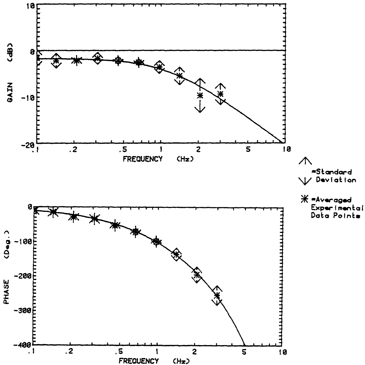
Figure 7-8 (a) OCCULOMETER WITH FEEDBACK AZIMUTH CLOSED LOOP 9 Deg. Maximum Field For 6 Subjects, 6 Runs
