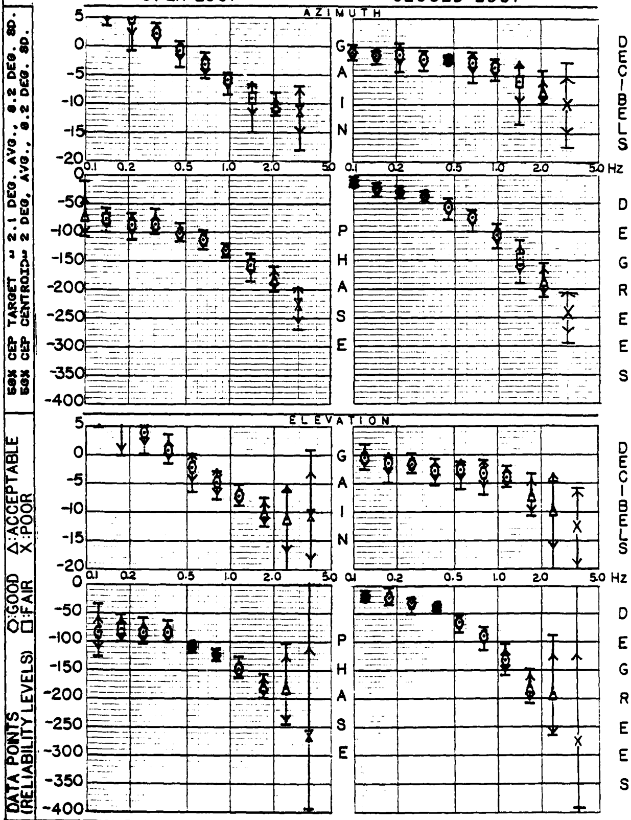
FREQ. RESP. STATISTICS OF 60CULOM. WITH FB RUNS ON 6 SUBJECTS AT 6 DEG. MAX. FIELD OPEN LOOP CLOSED LOOP
