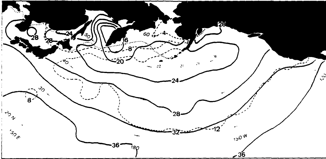
Figure 19a. January 0000 GMT mean surface visibility (km) (solid lines), standard deviations at 4 km (dashed lines), maximum southern extent of ice coverage .1 or greater (dotted line), (U.S. Naval Weather Service Environmental Detachment, 1977).
