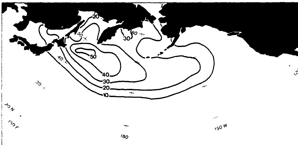
Figure 9b. Same as 9a for 1200 GMT.
