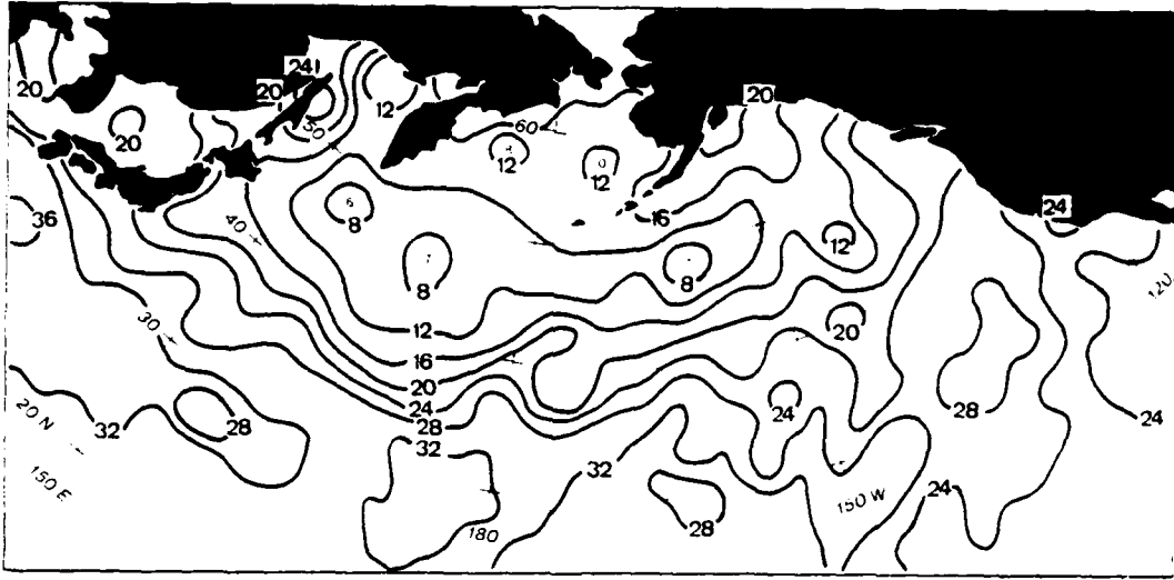
Figure 6a. July 0900 GMT mean surface visibility (km).
