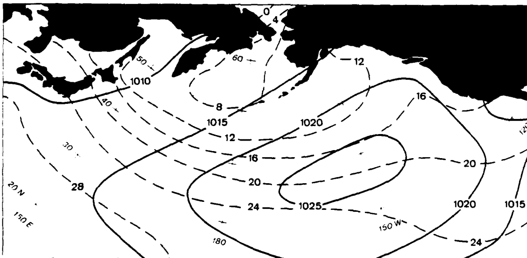
Figure 7b. July mean sea-level pressure (mb) (solid lines) and mean sea-surface temperatures ( ^{\circ}\text{C} ) (dashed lines) for the North Pacific Ocean, (U.S. Naval Weather Service Environmental Detachment, 1977).
