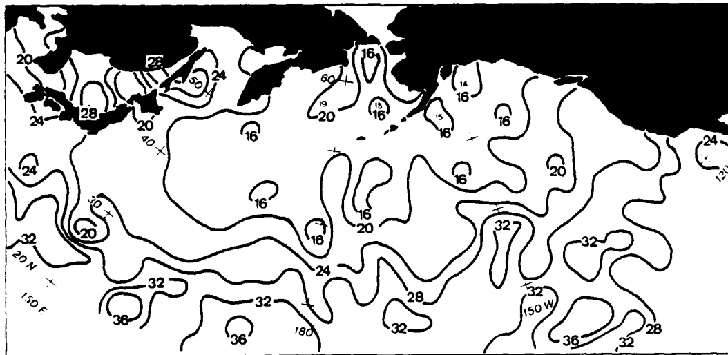
Figure 26b. April 0900 GMT mean surface visibility (km).
