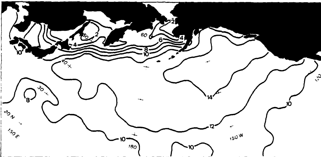
Figure 20b. January 0000 GMT standard deviations of surface visibility (km).
