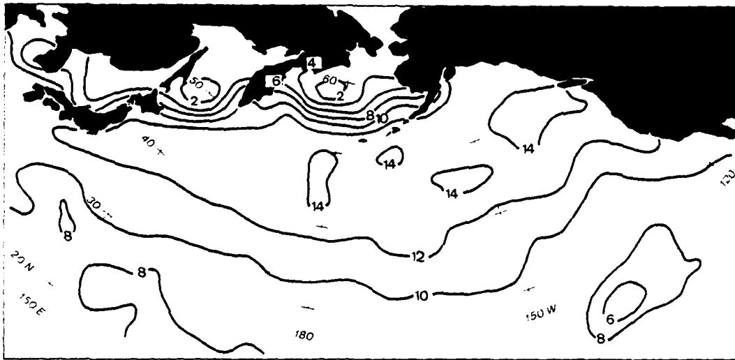
Figure 16a. October 0000 GMT standard deviations of mean surface visibility (km).
