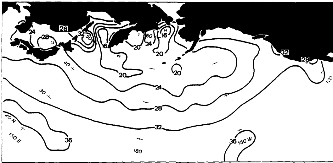
Figure 27a. April 1200 GMT mean surface visibility (km).
