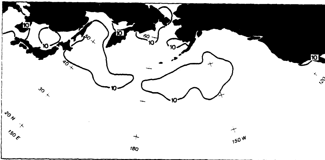
Figure 28b. April frequency of fog occurrence (%).
