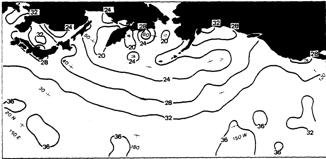
Figure 15b. Same as 15a for 1200 GMT.
