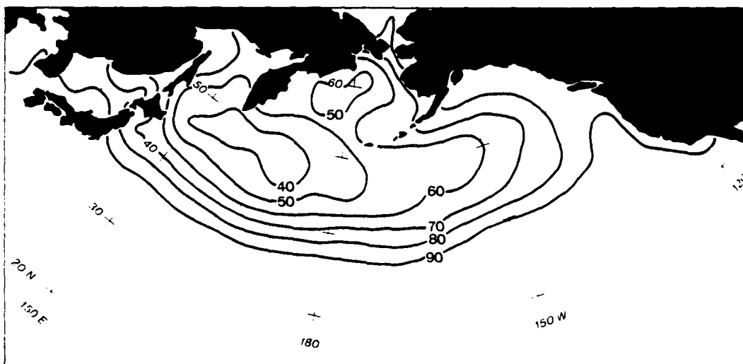
Figure 12b. Same as 12a for 1200 GMT.
