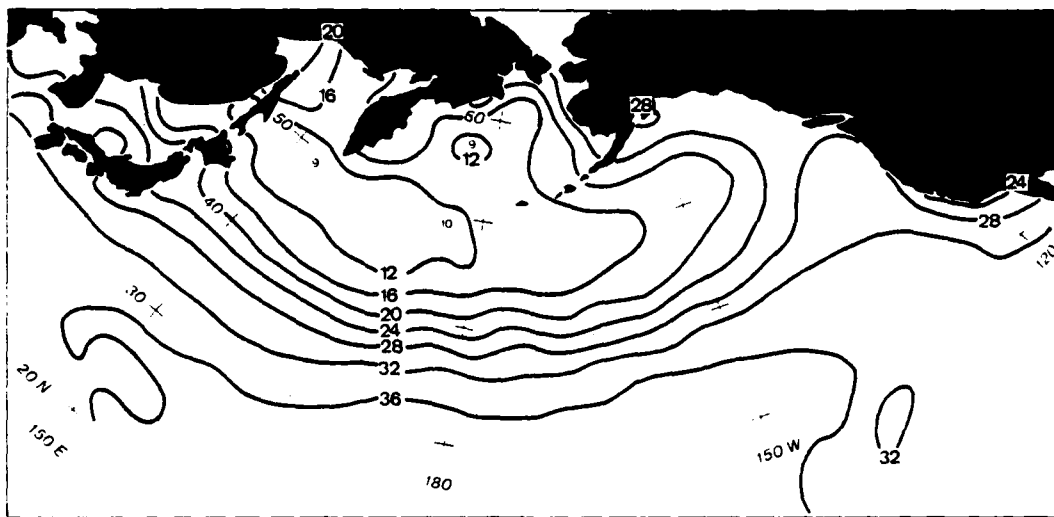
Figure 8b. Same as 8a for 1800 GMT.
