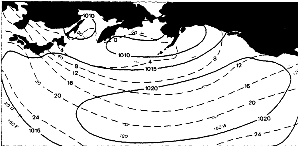
Figure 28a. April mean sea-level pressure (mb) (solid lines), mean sea-surface temperatures (°C) (dashed lines) for the North Pacific Ocean, (U.S. Naval Weather Service Environmental Detachment, 1977).
