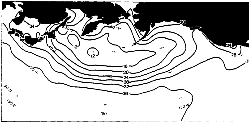
Figure 8a. July 0600 GMT mean surface visibility (km).
