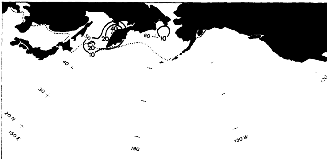
Figure 22a. January 1200 GMT frequency of visibility less than 2 km (solid lines) (%), maximum southern extent of ice coverage .1 or greater (dotted line), (U.S. Naval Weather Service Environmental Detachment, 1977).
