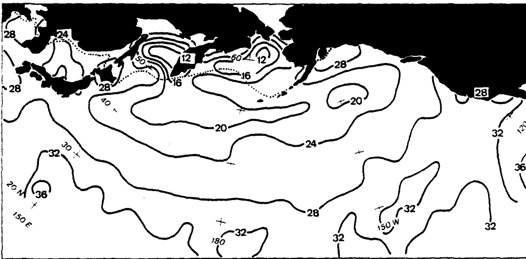
Figure 25b. Same as 25a for 0130 LST.
