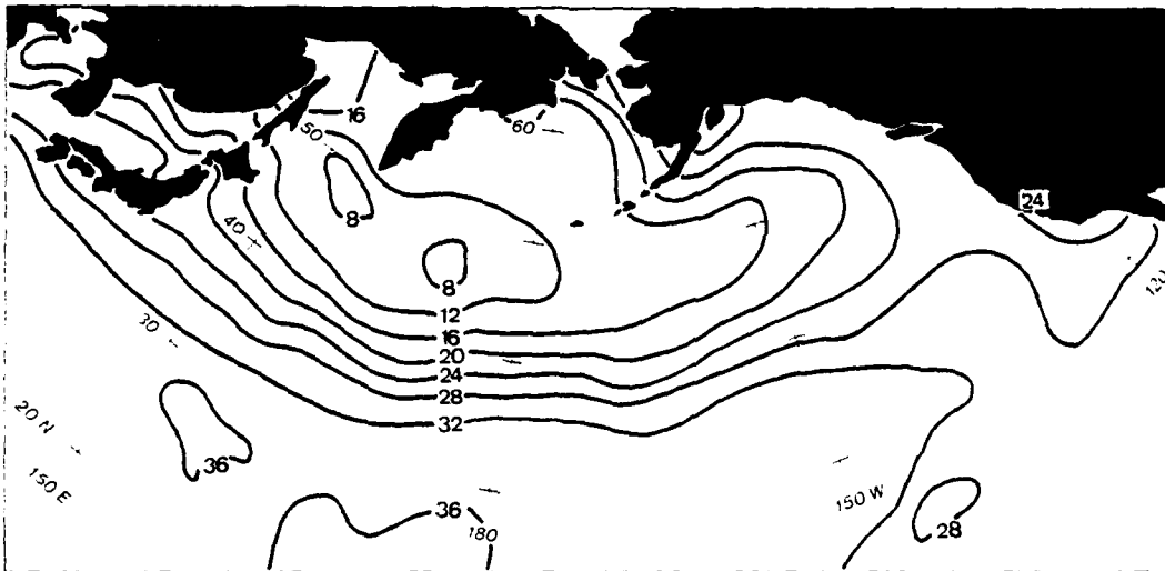
Figure 14a. July 0130 LST mean surface visibility (km).
