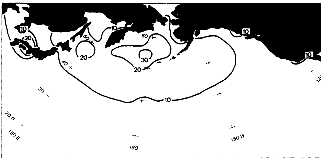
Figure 11a. July 0000 GMT frequency of visibility equal to or greater than 2 km and less than 10 km (%).
