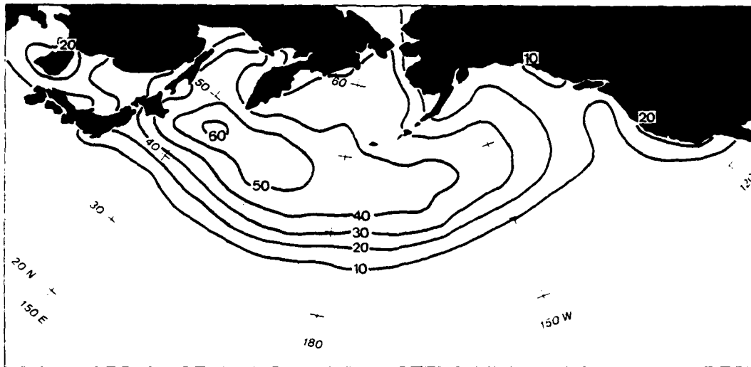
Figure 13a. July frequency of fog occurrence (%).
