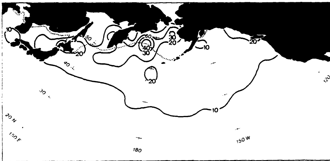
Figure 22b. January 0000 GMT frequency of visibility equal to or greater than 2 km and less than 10 km (solid lines) (%), maximum southern extent of ice coverage .1 or greater (dotted line), (U.S. Naval Weather Service Environmental Detachment, 1977).
