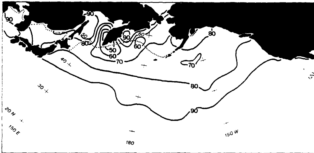
Figure 23b. January 0000 GMT frequency of visibility equal to or greater than 10 km (solid lines) (%), maximum southern extent of ice coverage .1 or greater (dotted line), (U.S. Naval Weather Service Environmental Detachment, 1977).
