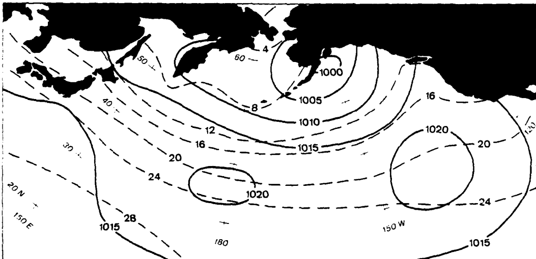
Figure 16b. October mean sea-level pressures (mb) (solid lines) and sea-surface temperatures ( ^{\circ}\text{C} ) (dashed lines) for the North Pacific Ocean, (U.S. Naval Weather Service Environmental Detachment, 1977).
