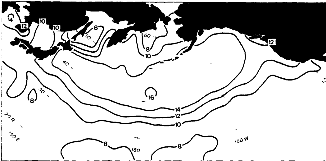
Figure 7a. July 0000 GMT standard deviations of surface visibility (km).
