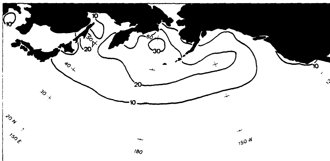
Figure 11b. Same as 11a for 1200 GMT.
