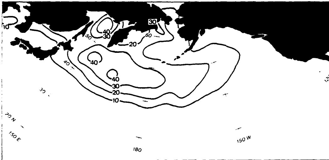
Figure 9a. July 0000 GMT frequency of visibility less than 2 km (%).
