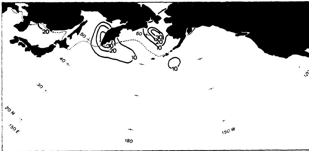
Figure 21b. January 0000 GMT frequency of visibility less than 2 km (solid lines) (%), maximum southern extent of ice coverage .1 or greater (dotted line), (U.S. Naval Weather Service Environmental Detachment, 1977).
