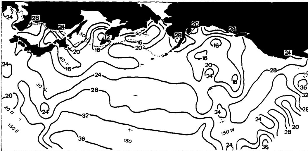
Figure 25a. January 0000 LST mean surface visibility analysis (km) (solid lines), maximum southern extent of ice coverage .1 or greater (dotted line), (U.S. Naval Weather Service Environmental Detachment, 1977).
