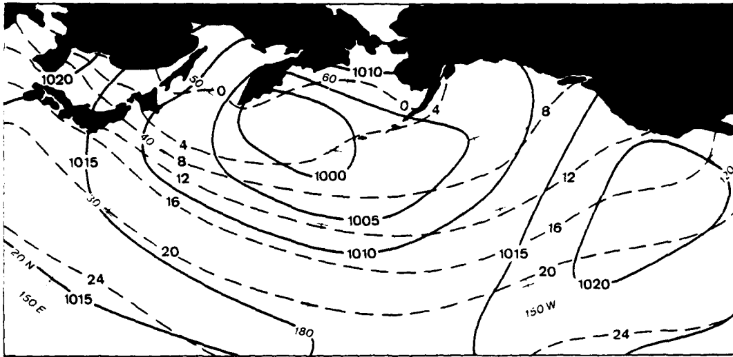
Figure 21a. January mean sea-level pressures (mb) (solid lines), sea-surface temperatures ( ^{\circ} C) (dashed lines) for the North Pacific Ocean, (U.S. Naval Weather Service Environmental Detachment, 1977).
