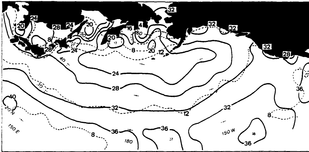
Figure 26a. April 0000 GMT mean surface visibility (km) (solid lines), standard deviations at 4 km intervals (dashed lines).
