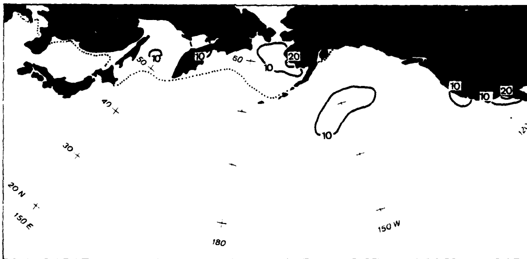
Figure 24b. January frequency of fog occurrence (solid lines) (%), maximum southern extent of ice coverage .1 or greater (dotted line), (U.S. Naval Weather Service Environmental Detachment, 1977).
