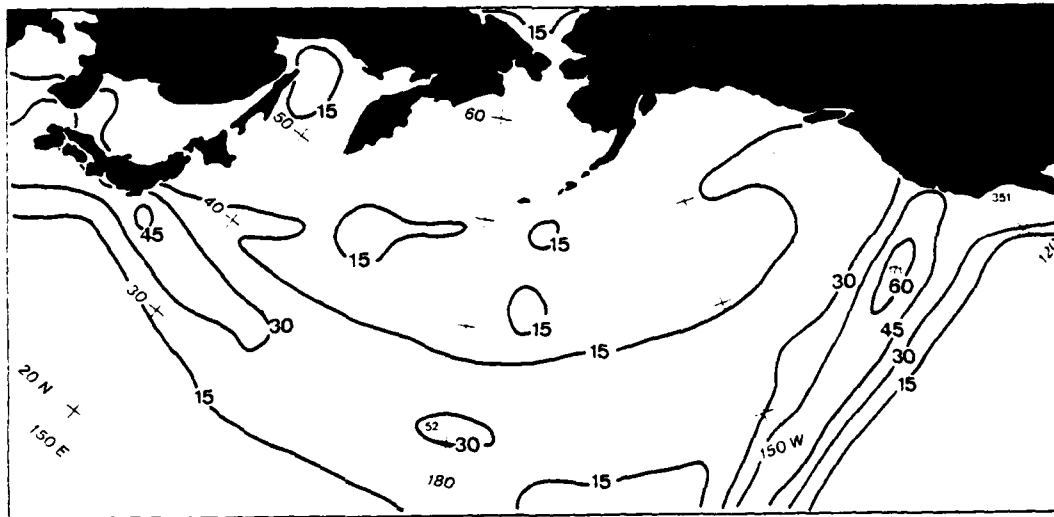
Figure 18b. Same as 18a for 1200 GMT.
