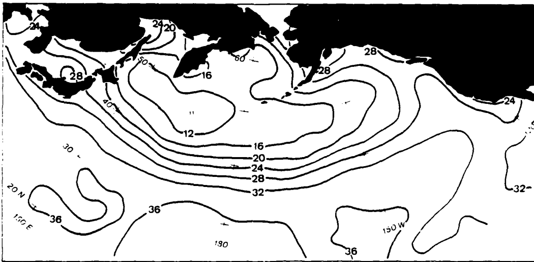
Figure 6b. Same as 6a for 1200 GMT (km).
