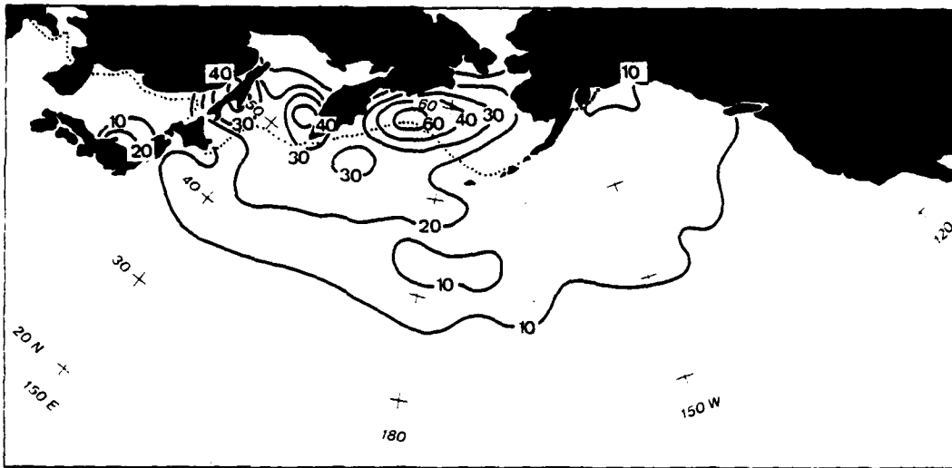
Figure 23a. January 1200 GMT frequency of visibility equal to or greater than 2 km and less than 10 km (solid lines) (%), maximum southern extent of ice coverage .1 or greater (dotted line), (U.S. Naval Weather Service Environmental Detachment, 1977).
