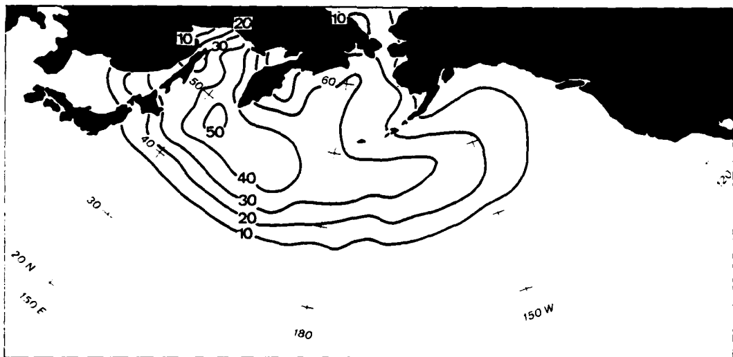
Figure 10b. Same as 10a for 1800 GMT.
