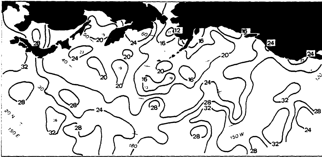
Figure 15a. October 0900 GMT mean surface visibility (km).
