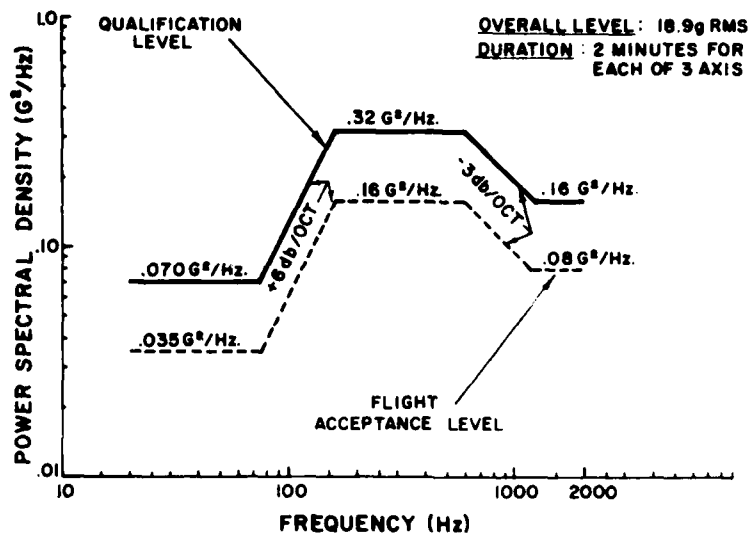
Figure 34: Random vibration input to S/N 2 cold finger.
