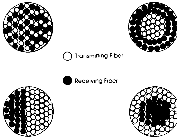
Figure 36: Photonic sensor fibers.
