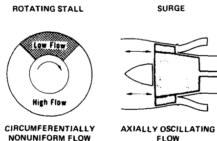
FIG. 11.—Sketch of Two Possible Modes of Compressor Instability
