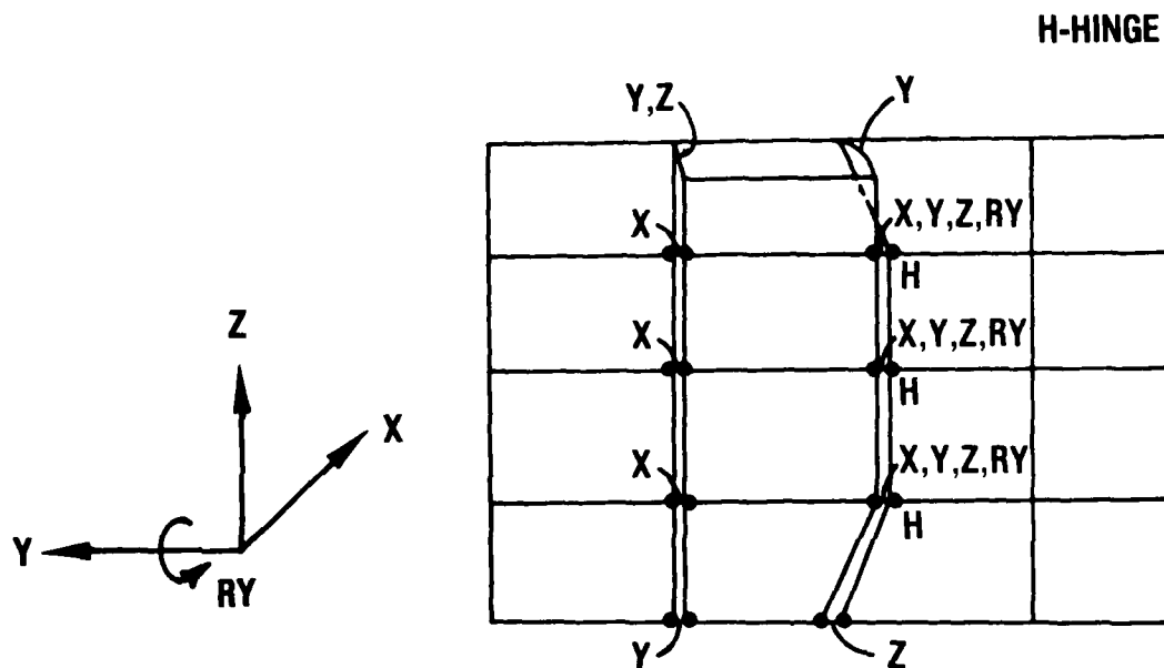
Figure 8. Case 2. Personnel door endwall, connected degrees of freedom between door and doorframe.
