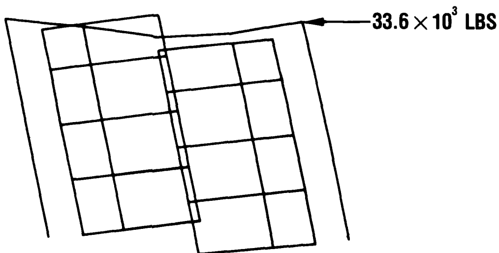
Figure 16. Case 5. Cargo door endwall, deformed body plot.
