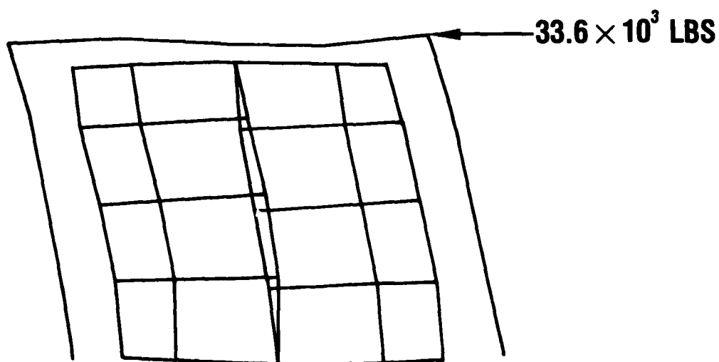
Figure 23. Case 9. Cargo door endwall, connected degrees of freedom between door and doorframe.
