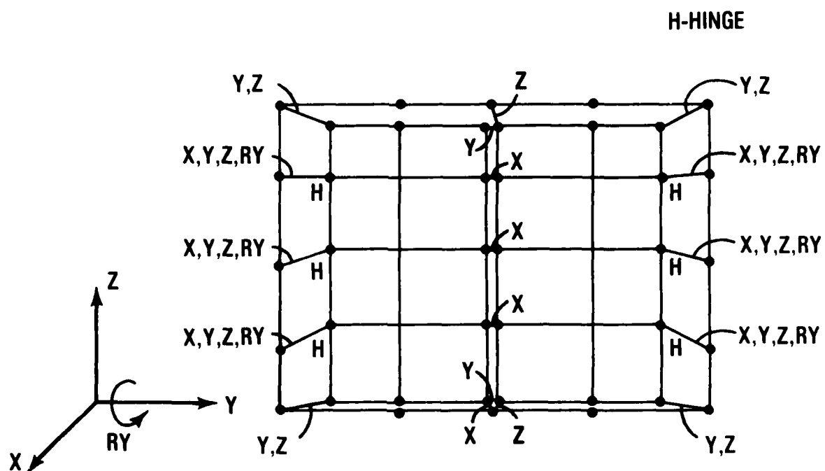
Figure 15. Case 5. Cargo door endwall, connected degrees of freedom between door and doorframe.
