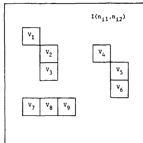
Figure 2.2 Third-order Statistics
