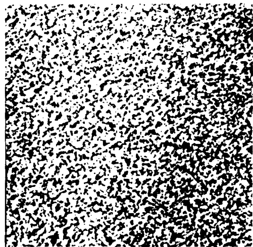
(d) Second-order Linear Model with Non-stationary Noise
