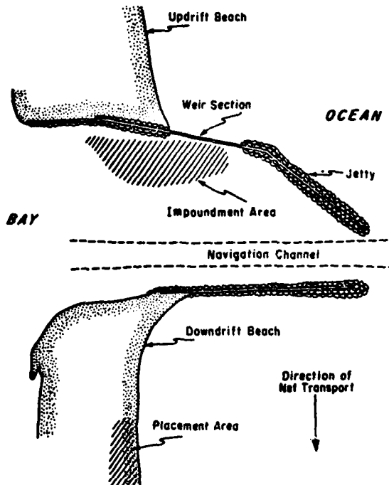
Figure 4. Weir jetty with impoundment area between jetties.
