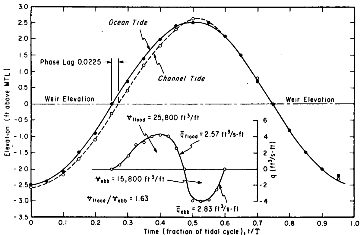
Figure 15. Discharge over weir as a function of time during a tidal cycle (weir 1.5 feet below MTL).
