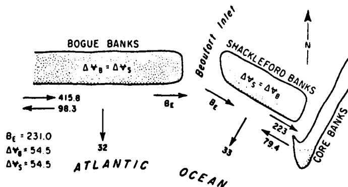
Figure 27. Weir-jetty construction sediment budget for strategy 3.
