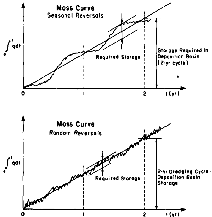
Figure 31. Longshore transport mass curves for a site where reversals are seasonal and a site where reversals are random.
