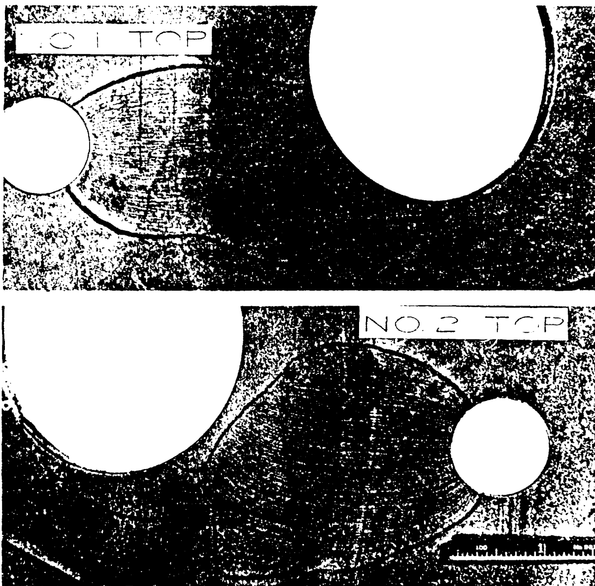
Figure 3. Strain patterns in brittle lacquer on top surface of mortar baseplate; note direction of strain pattern.
