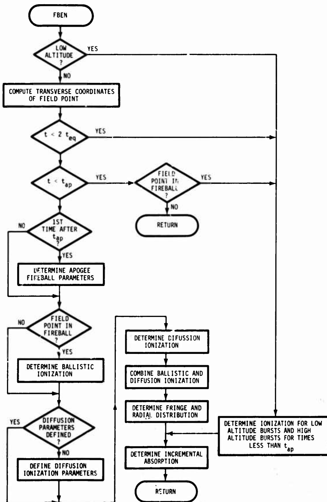
Figure 13. Flowchart for subroutine FBEN.
