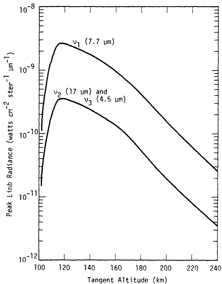
Figure C-3. Estimated peak spectral limb radiance in the \nu_1 , \nu_2 , and \nu_3 bands of \text{N}_2\text{O} excited by earthshine scatter at 3 sec following a megaton-class high-altitude nuclear burst.
