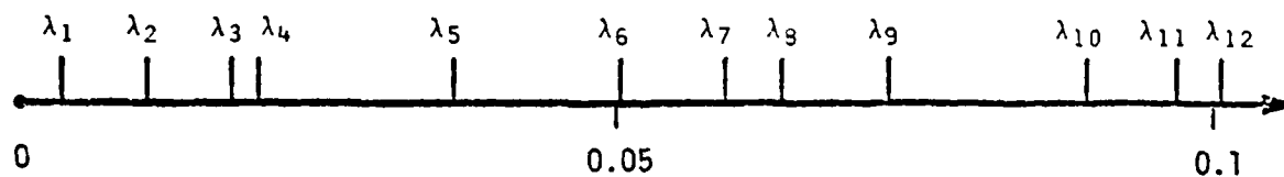
Figure 1b. Eigenvalues of the above system.
