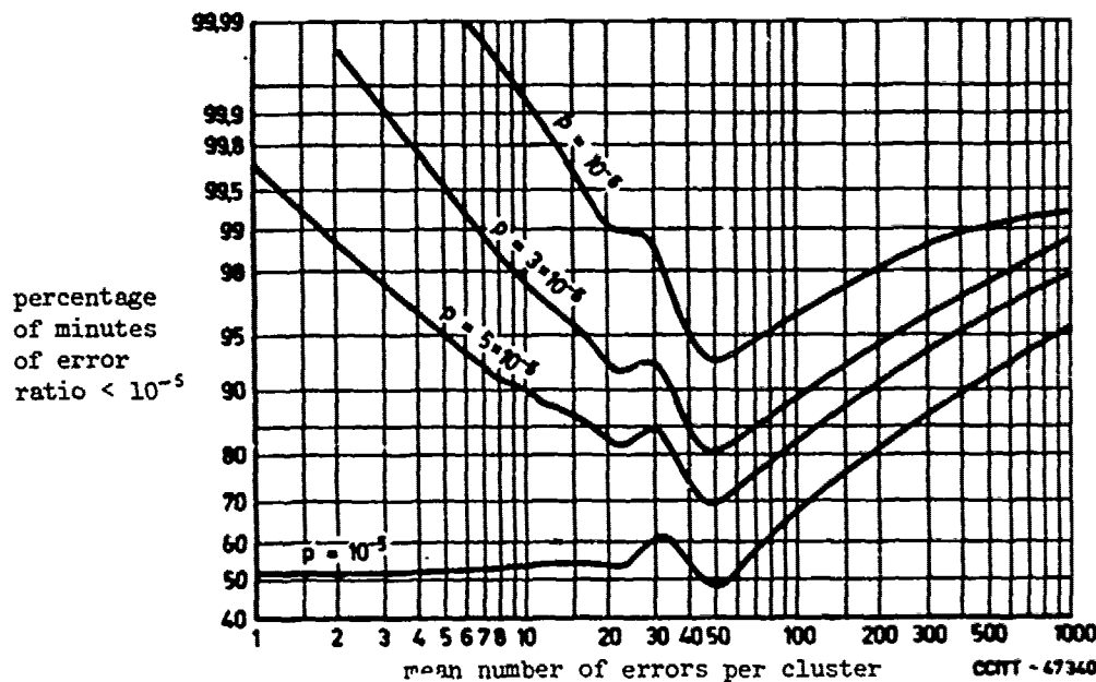
Figure 2 - The variation with degree of clustering of the percentage of minutes of 64 kbit/s transmission having an error ratio less than 10^{-5} for different values of long-term mean error ratio ( p )
