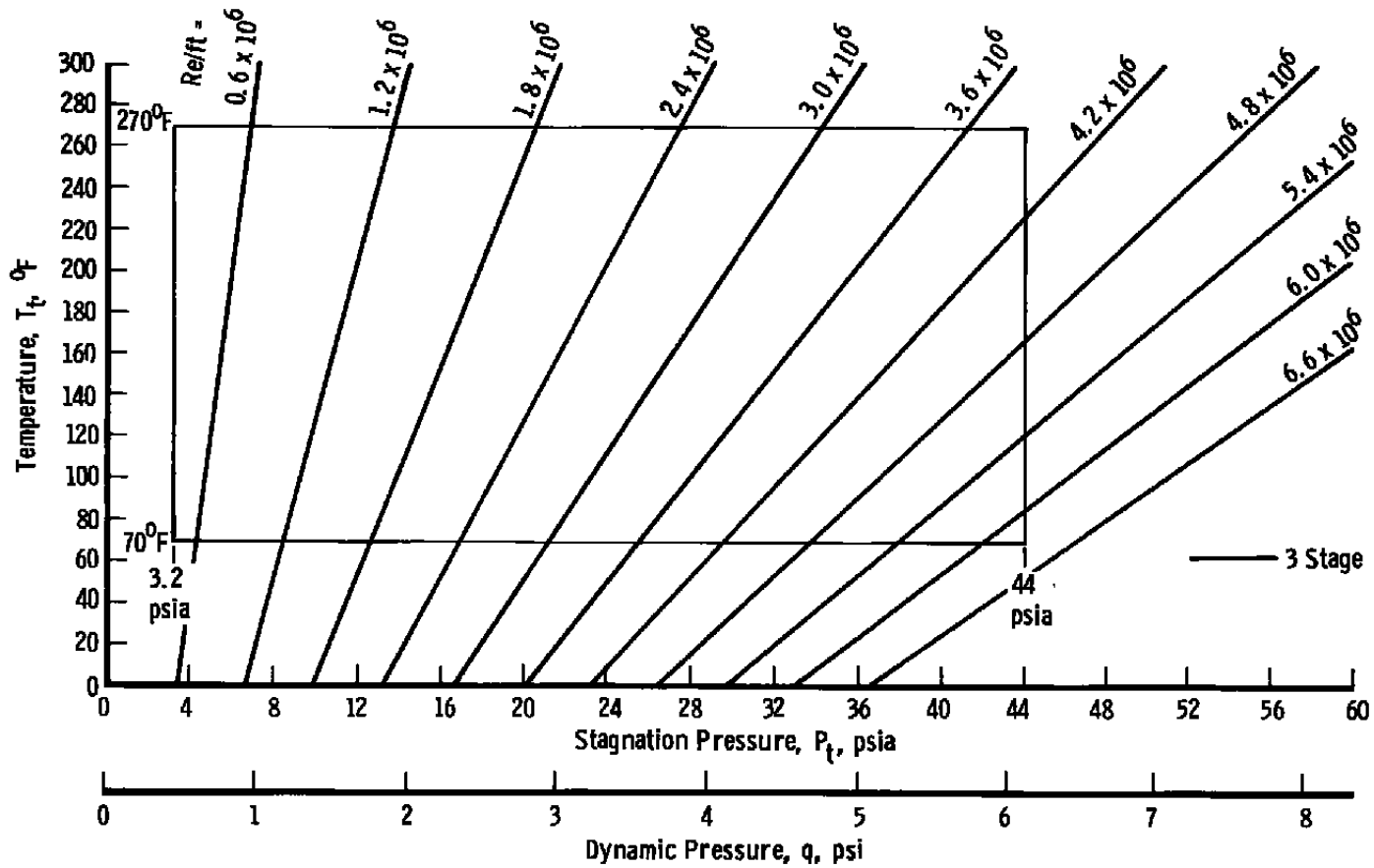
h. M = 3.25 Figure A-6. Continued.
