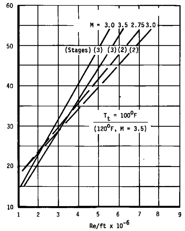
Figure A-10. Electrical usage for Tunnel A.
