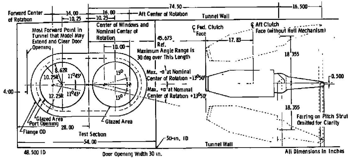
c. Test section (elevation), Tunnel C Figure C-1. Concluded.
