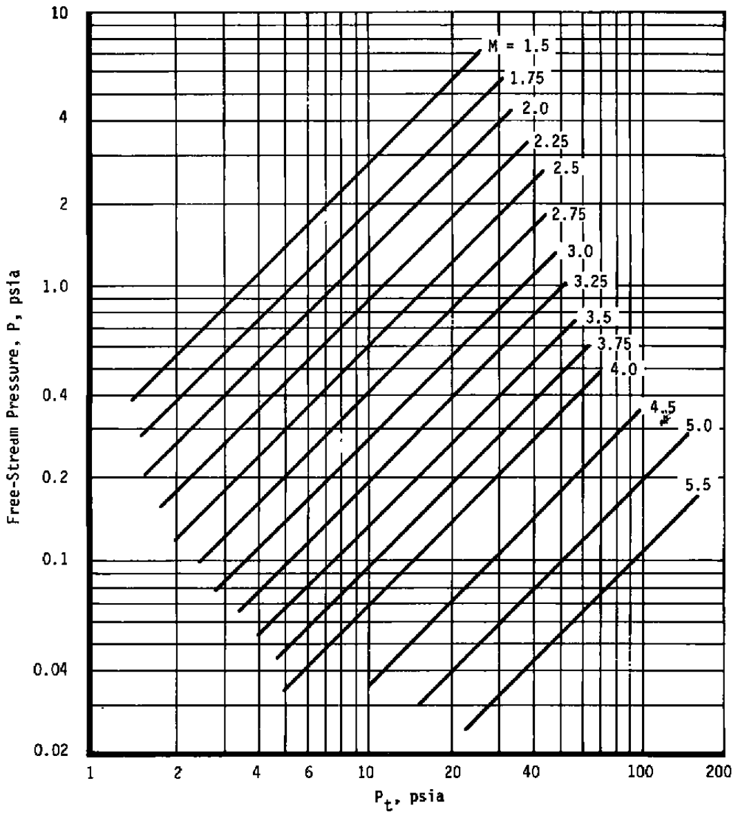
Figure A-8. Free-stream pressure, Tunnel A.
