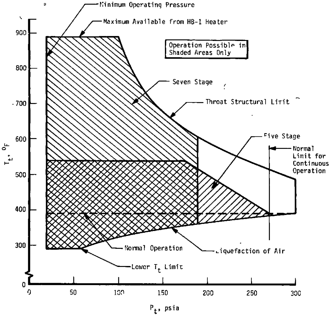
c. Closed circuit for expanded envelope Figure B-7. Concluded.
