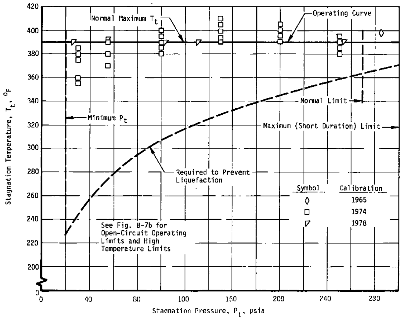
a. Normal operating envelope Figure B-7. Stagnation conditions, Tunnel B – Mach 6.
