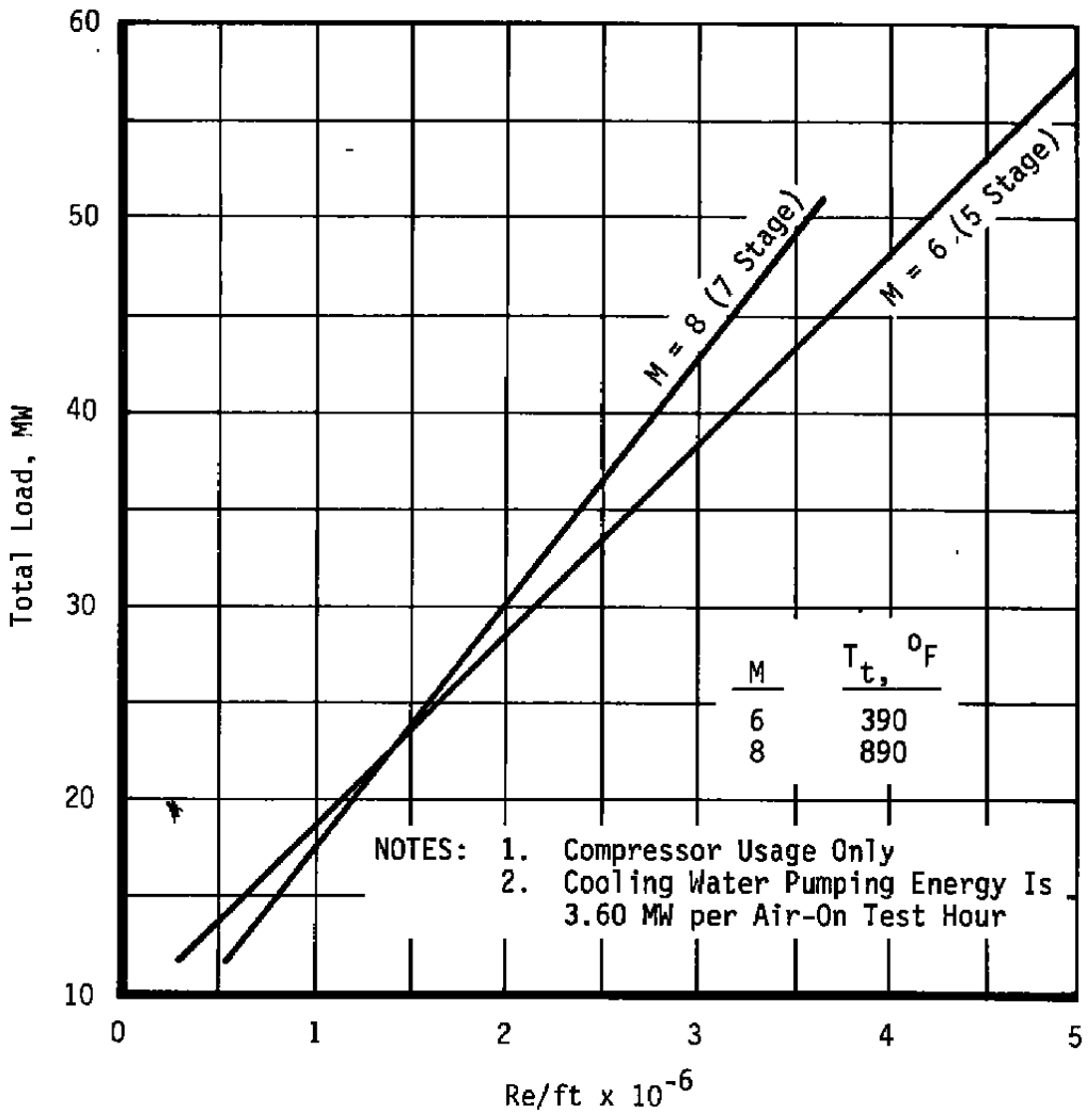
Figure B-24. Electrical usage for Tunnel B.
