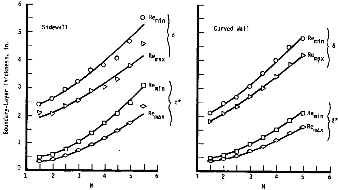
b. Tunnel A boundary-layer and displacement thickness Figure A-2. Concluded.
