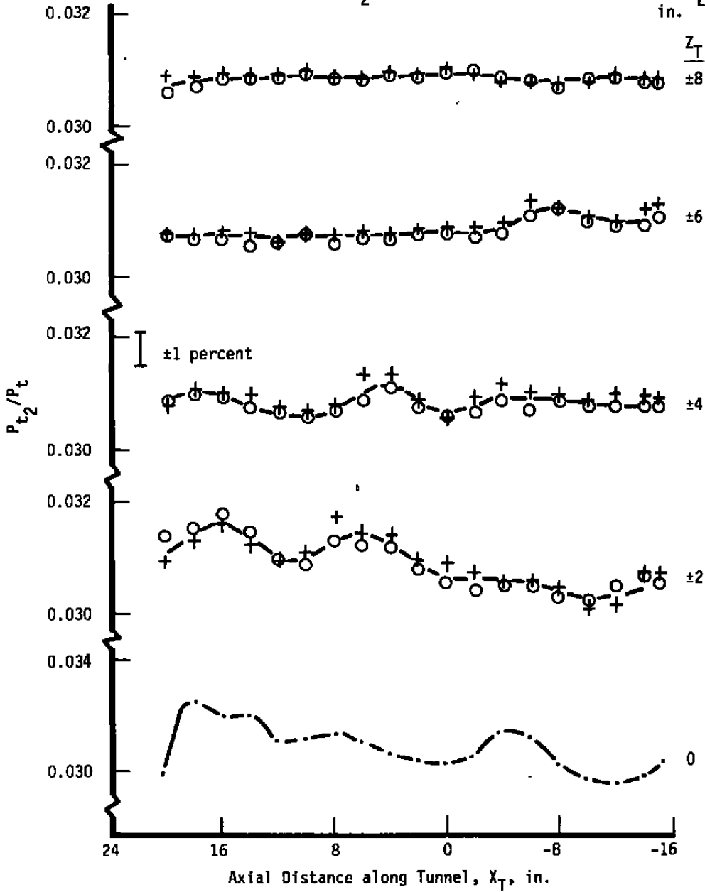
Figure B-5. Axial pitot pressure distributions, Tunnel B — Mach 6.
