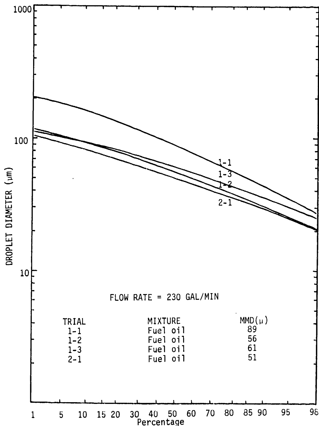
Figure 2-2 Cumulative Mass Distribution of Droplets as a function of Droplet-Diameter
