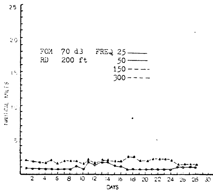
Figure 40 Median detection range (MDR) versus time for the ODT-FACT analysis: FOM of 70 dB, receiver depth of 200 feet, frequency range of 25 Hz, 50 Hz, 150 Hz, 300 Hz.
