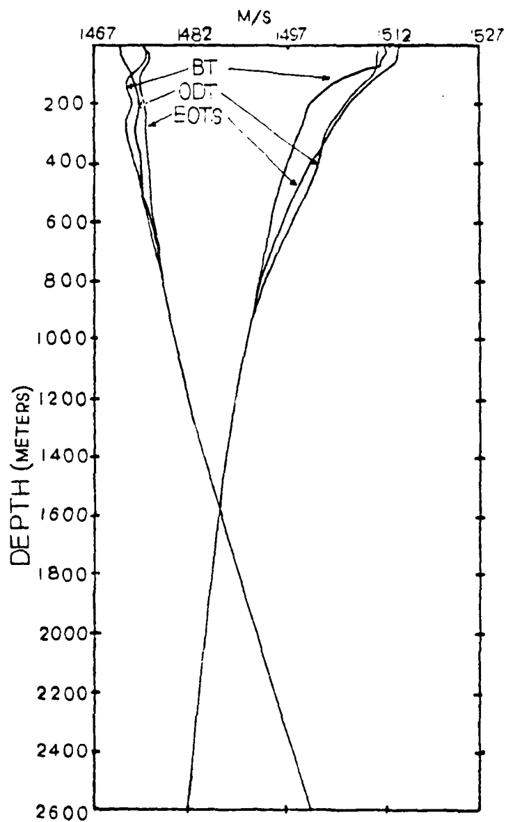
Figure 84 "Average" thermal structure and sound velocity profiles for May 1980, for BT, ODT, and EOTS analyses.
