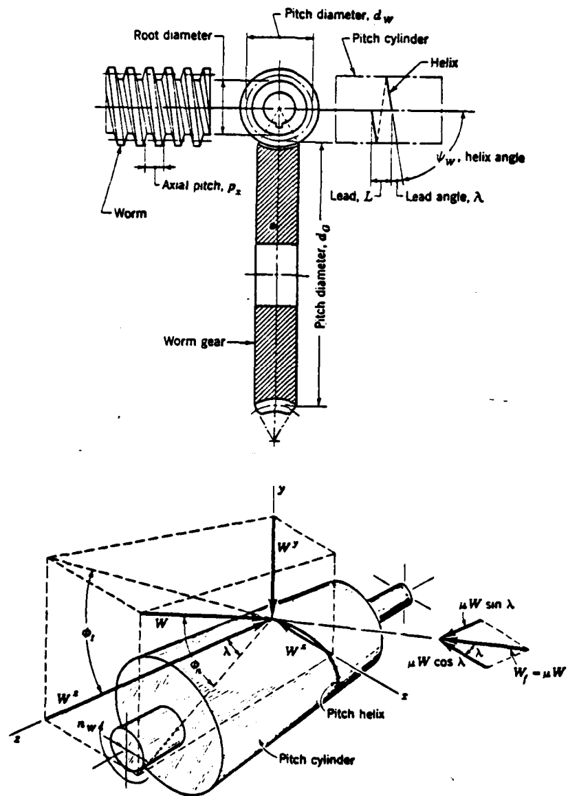
Figure 15. Worm and Worm Gear Nomenclature
