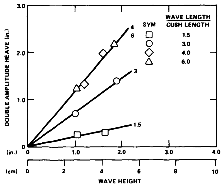
Figure 3.5.18a - Froude Number = 1.72
