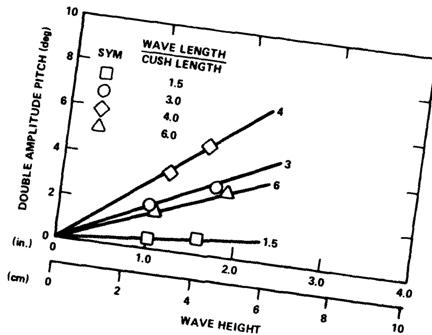
Figure 3.5.17a - Froude Number = 1.72
