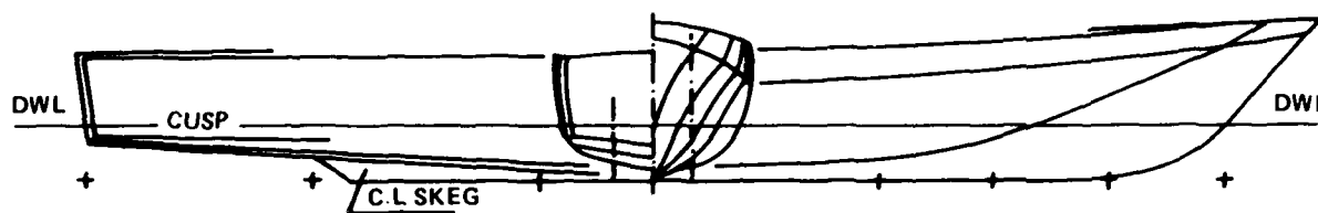
Figure 3.2.1 - Typical Body Plan of a Round-Bilge Hull
