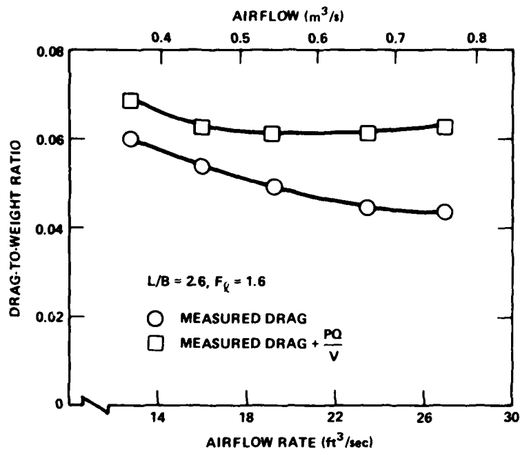
Figure 3.5.7 - Effect of Airflow Rate on Drag
