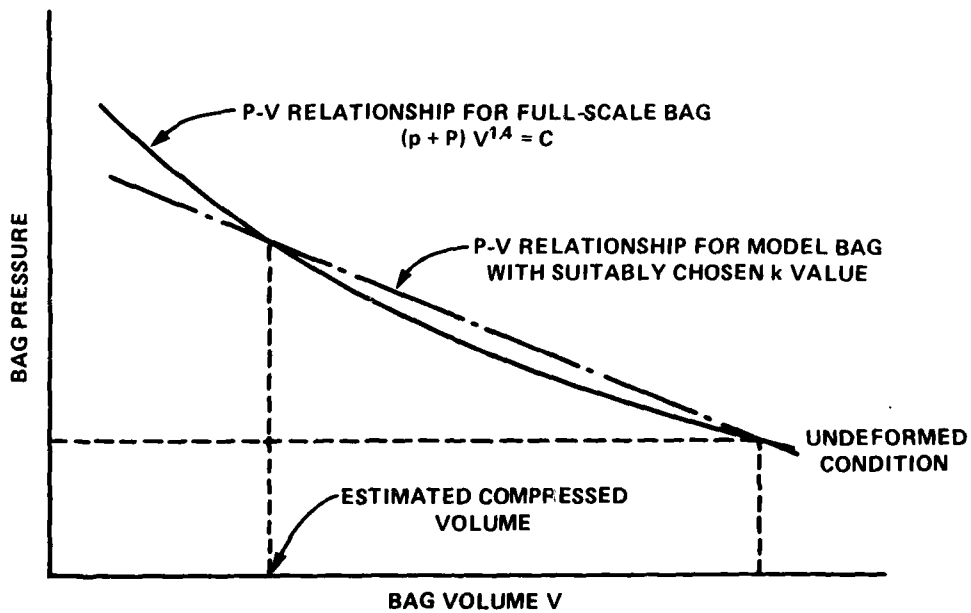
Figure 3.6.5b - Example of Pressure Volume Relationship
