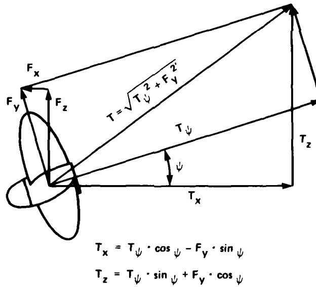
Figure 3.2.7 - Forces at Propeller in Oblique Flow
