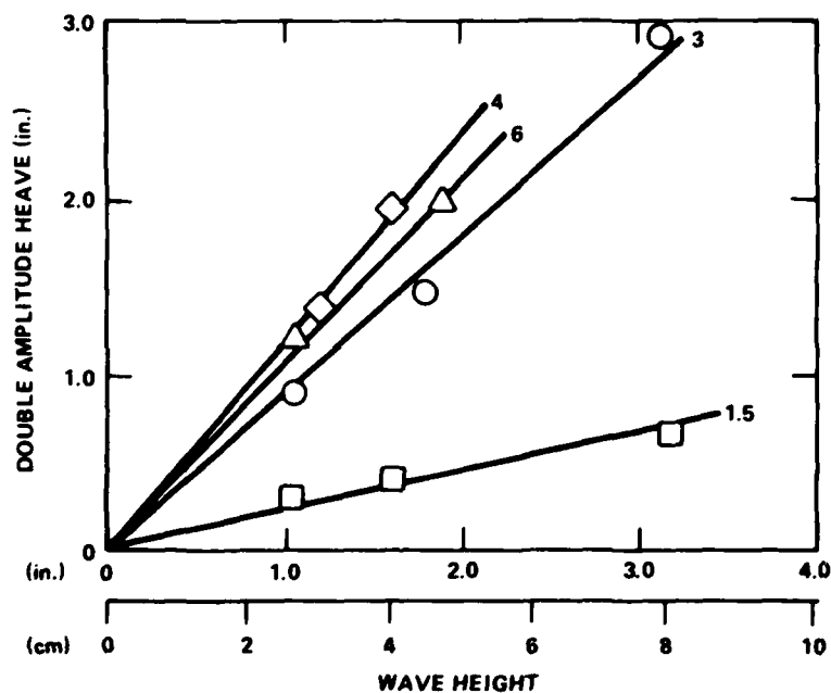
Figure 3.5.18b - Froude Number = 1.28
