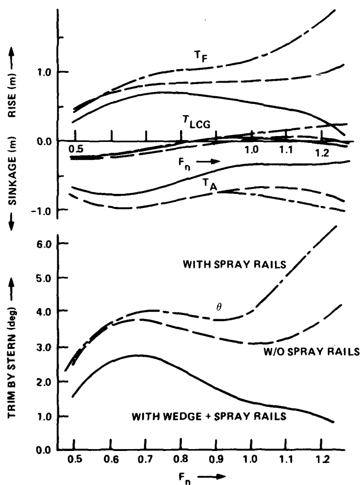
Figure 3.2.2 - Trim Variations
