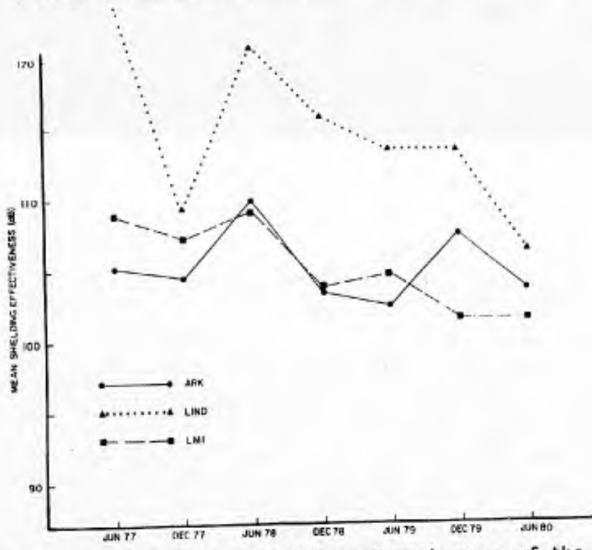
Figure 23. Comparison of the shielding effectiveness of the three room types versus aging (1 MHz frequency).
