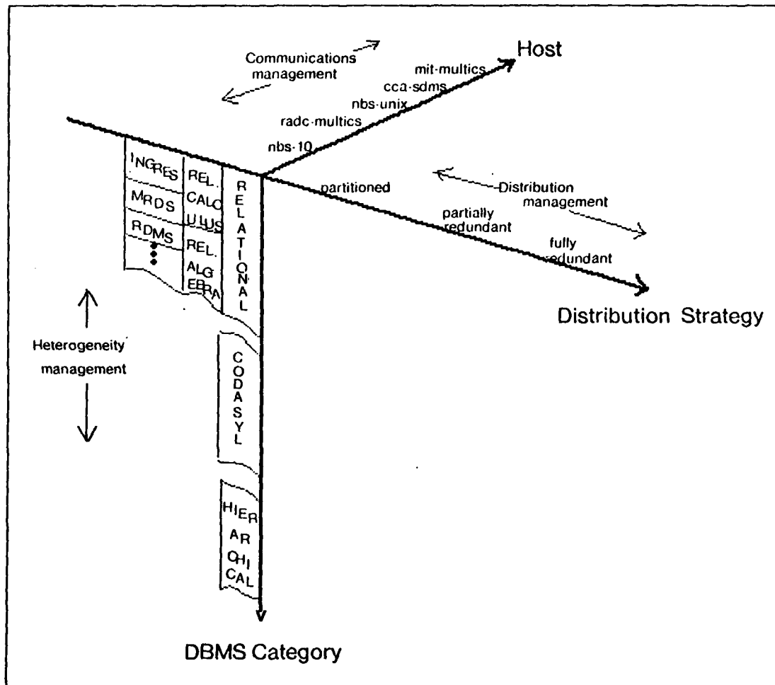
Figure 3. Dimensions of Variation of Database Systems
