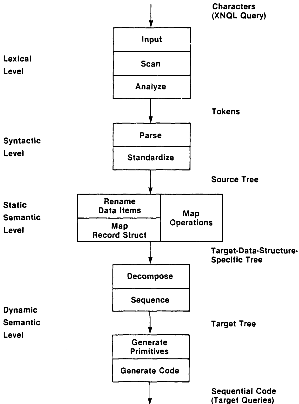
FIGURE 13. THE XNQL TRANSLATOR AS A TREE TRANSFORMER
