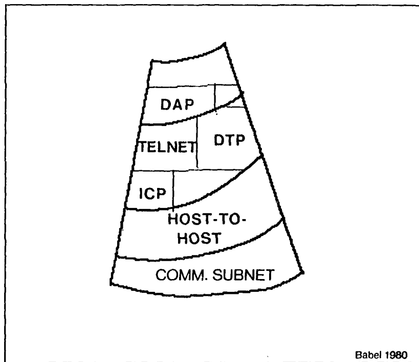
Figure 2. DAP as a Member of the Protocol Hierarchy
