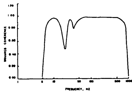
b. COHERENCE
