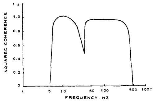
b. COHERENCE
