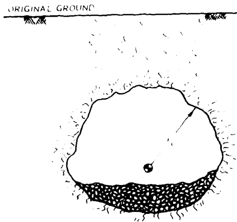
b. CAMOUFLET RESULTING FROM CONTAINED CHARGE
