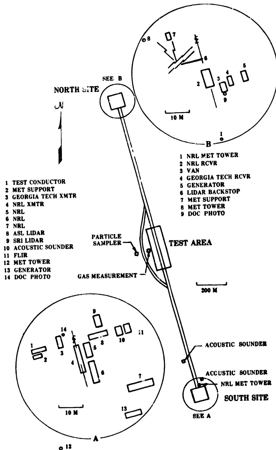
FIGURE 7.2 DETAILED LAYOUT OF DIRT-I SITE SHOWING LOCATIONS OF VANS AND EXPERIMENTS AT EACH END. PATH LENGTH FROM NORTH TO SOUTH IS 2 km. TEST AREA, WHERE EXPLOSIVES WERE DETONATED AND ARTILLERY SHELLS IMPACTED, IS 100 BY 300 m. REFERENCE [1].
