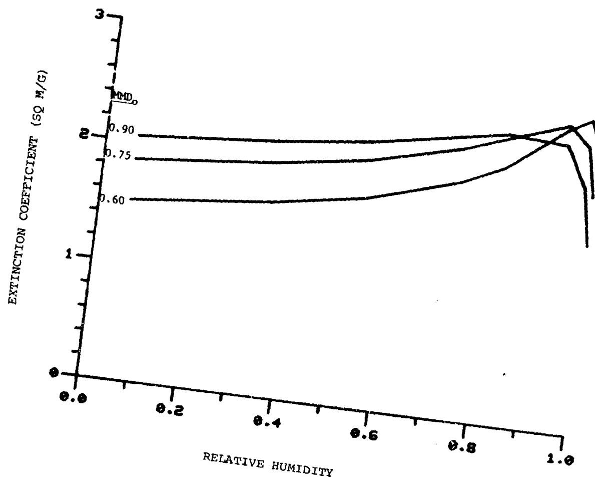
FIGURE 4.13 COMPUTED EXTINCTION COEFFICIENT FOR PHOSPHORUS SMOKES AT 1.06 \mu\text{m} WAVELENGTH VERSUS RELATIVE HUMIDITY. FRICKEL ET AL. [4].
