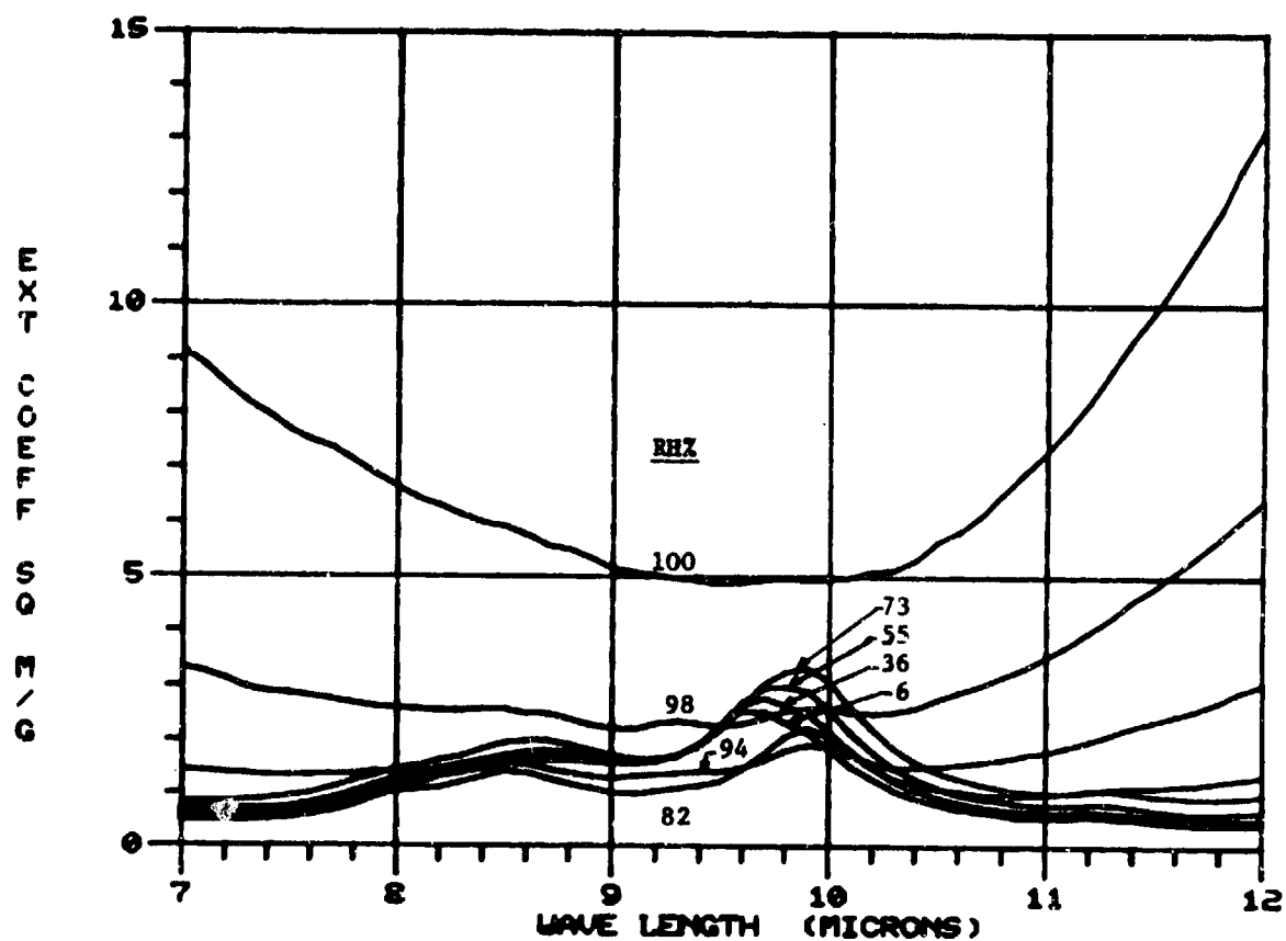
FIGURE 4.6 EXTINCTION COEFFICIENT FOR VARIOUS CONCENTRATIONS (RELATIVE HUMIDITY LEVELS) FOR PHOSPHORIC ACID IN THE FAR-IR. UNITS ARE m^2 PER GRAM OF PHOSPHORUS CONTAINED IN THE AEROSOL. FRICKEL ET AL. [4].
