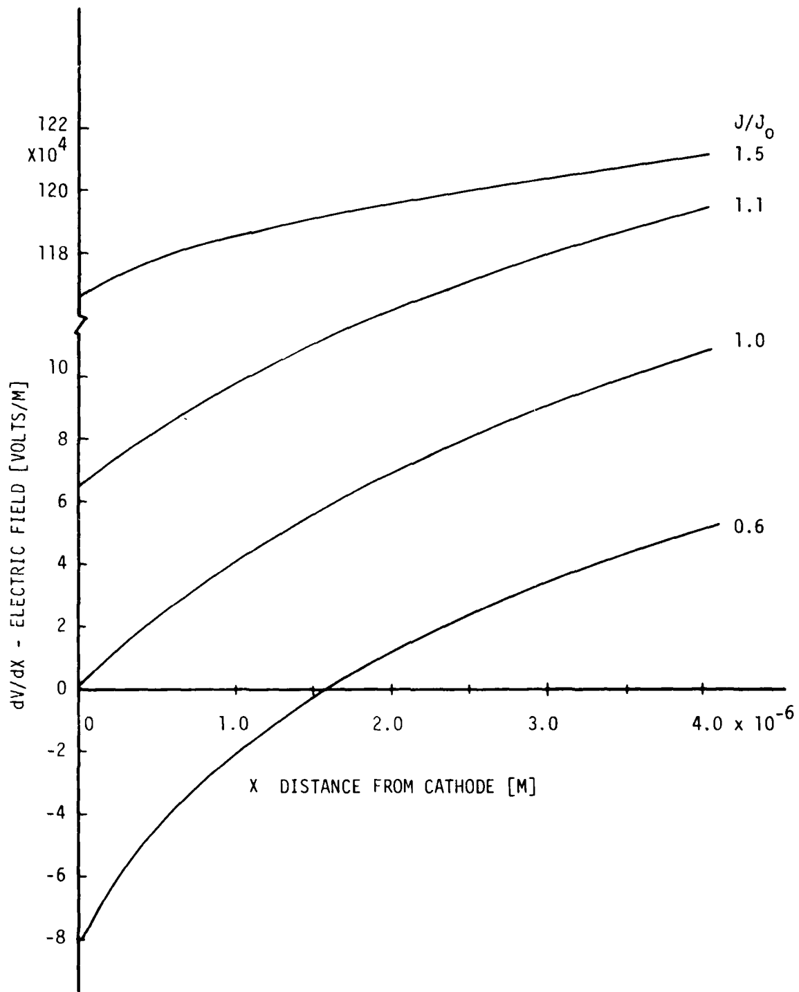
Figure 27. The Negative of the Electric Field.
