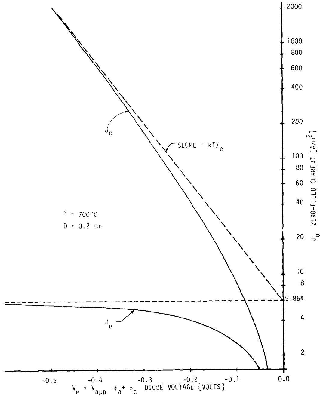
Figure 13. The Zero field Current J_0 and the Transition Current J_e Plotted as functions of the Transition Voltage V_e for D = 0.2\text{mm} , T = 700^\circ\text{C} .
