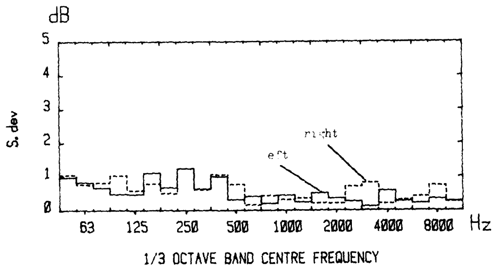
Fig 4 Mean attenuation spectra for earmuffs A, measured by objective methods
