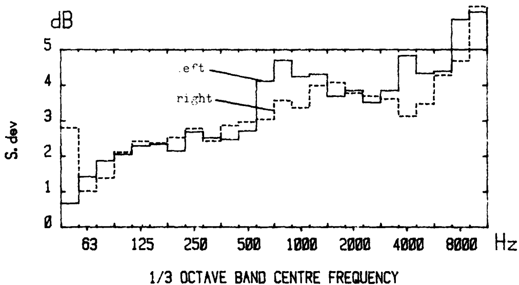
Fig 11 Mean attenuation spectra for earmuffs C, measured by semi-objective methods
