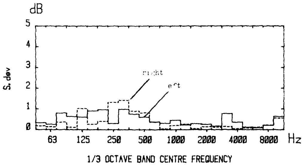
Fig 6 Mean attenuation spectra for earmuffs C, measured by objective methods
