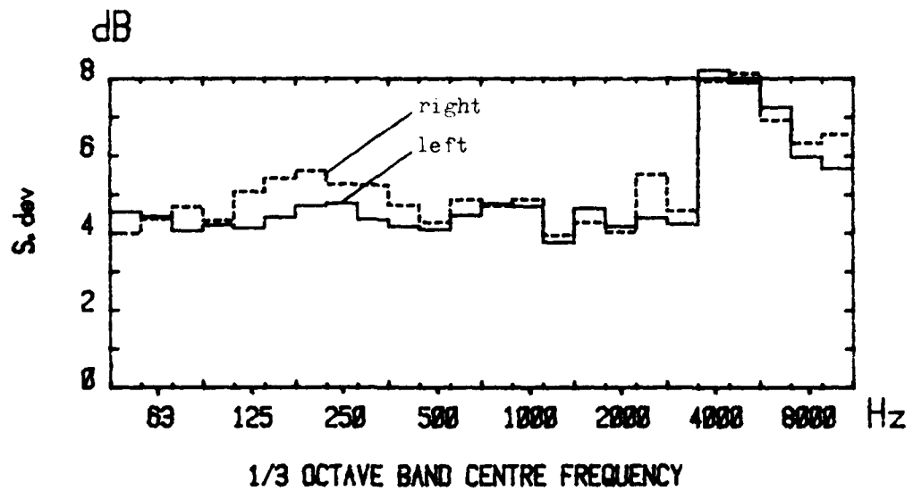
Fig A1 Mean attenuation spectra of earmuffs on standard headband
