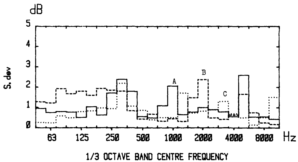
Fig 7 Comparison of mean attenuation spectra for each type of earmuff, measured by objective methods
