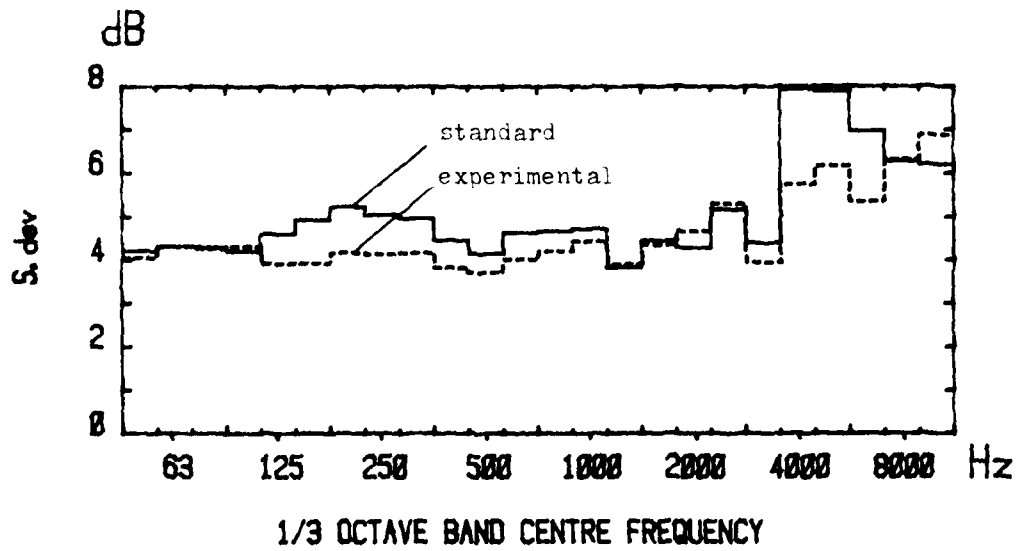
Fig A3 Comparison between the mean attenuation spectra for the two headbands
