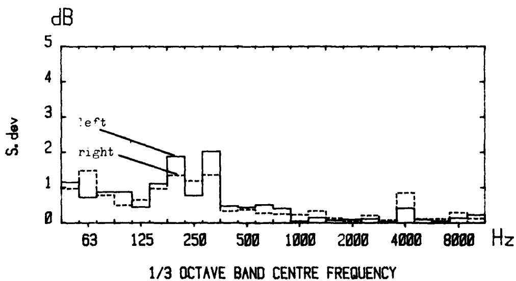
Fig 5 Mean attenuation spectra for earmuffs B, measured by objective methods
