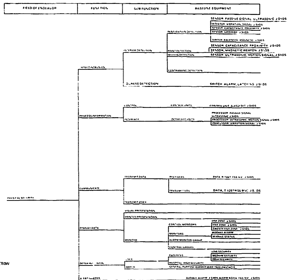
Figure VII-2. Baseline J-SIDS Equipment Summary for Physical Security VII-4
