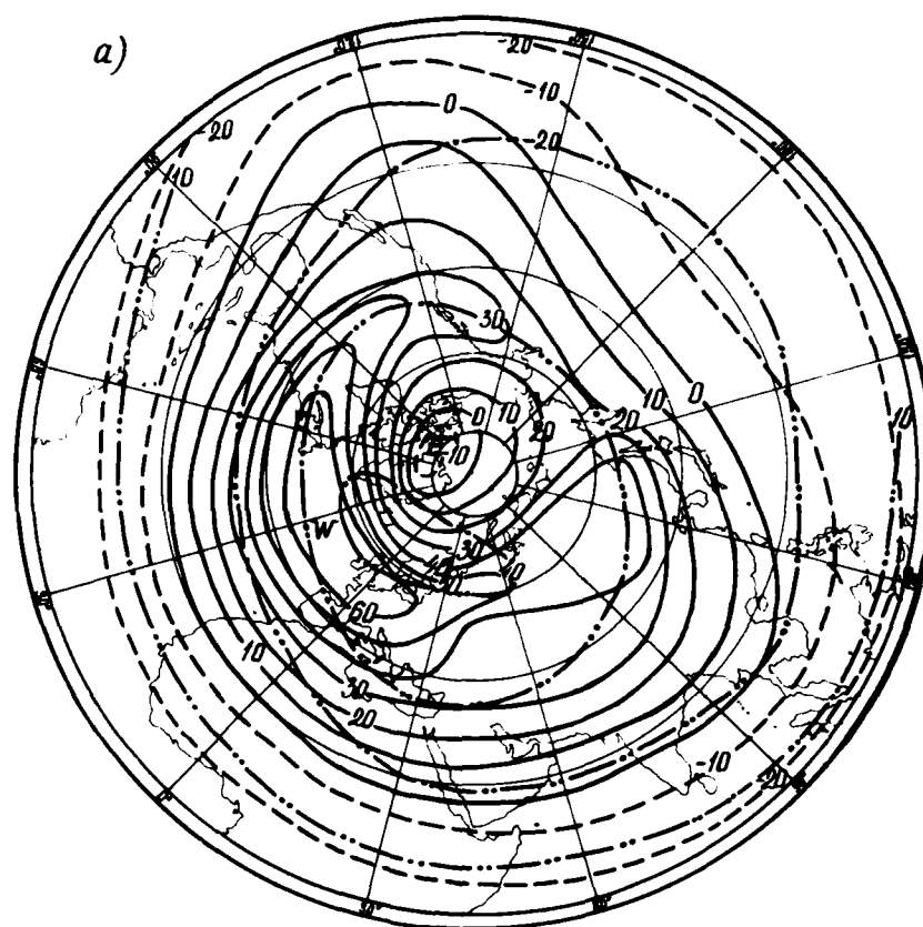
Fig.1. a) Chart of zonal wind mean montaly values and tueir standard deviations. January, 40 km level. Solid lines represent western wind component, dashed lines - eastern wind component, dash-dotted lines - standard deviations
