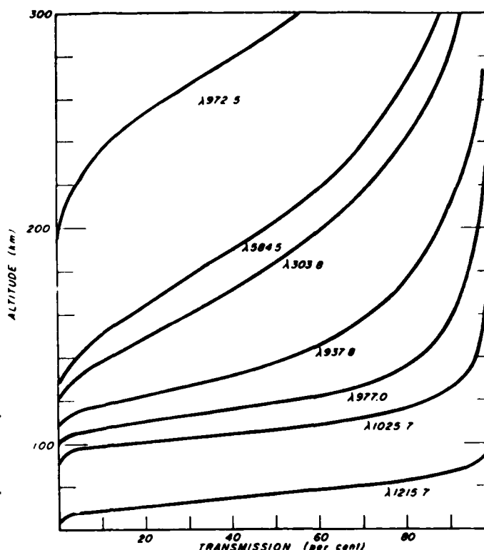
Fig. 6 NRL: XUV range atmospheric transmission curves published 1960[26].
