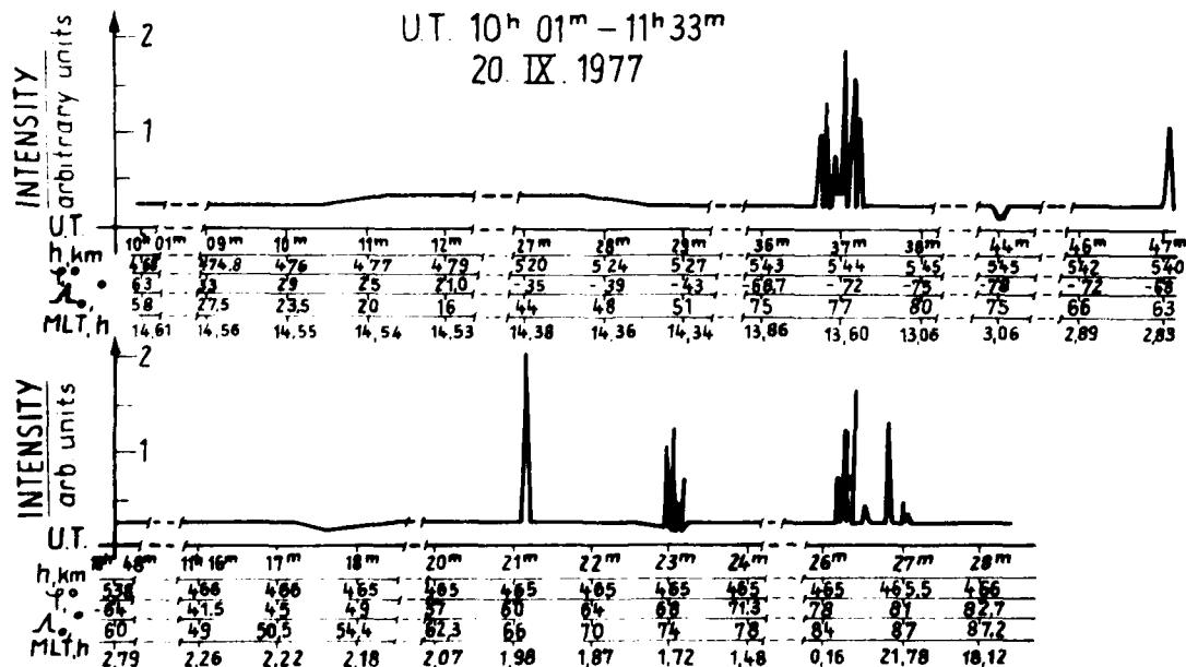
Fig. 1 Observations of aurora within the wavelength band 115 - 135 nm on September 20, 1977
