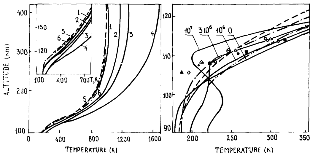
Fig.1a(left) The altitude temperature distributions for the theoretical and empirical models. The calculations are carried out for the altitude profile of K_h(z) characterized by K_h^{\max} = 10^8 \text{ cm}^2/\text{s} and z_m = 105 \text{ km} . 1 - vibrational excitation of NO( v=7 ) and CO 2 (01 6 0) in collisions NO-O and CO 2 -O is taken into account; 2 - no excitation in collisions NO-O; 3 - no excitation in collisions CO 2 -O; 4 - no excitation in collisions of O with both NO and CO 2 ; 5 - CIRA 72 model; 6 - Jacchia 1977 model. Fig.1b(right) The altitude temperature profiles in the lower thermosphere for varying values of K_h^{\max} at z_m = 105 \text{ km} . Also shown are: CIRA 72 model (dashed line), Jacchia 1977 model (dot-dashed line), measurements [13] (double-dot-dashed line), measurements [5] (open and solid circles, triangles and squares).
