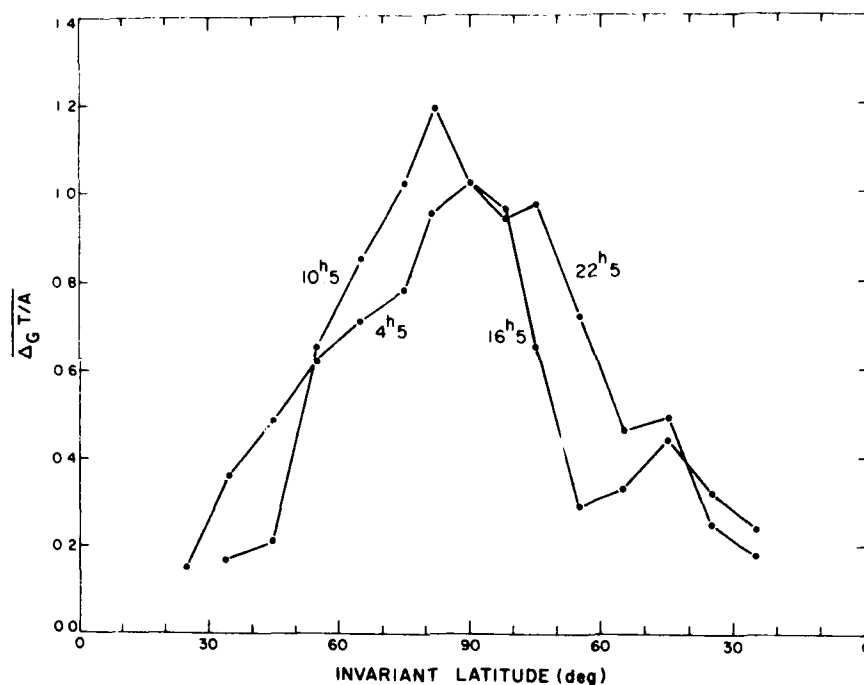
Fig. 2 Latitudinal profiles of \overline{\Delta G T/A} in the 10.5/22.5 and 4.5/16.5 meridional planes for K_p' in the range 3-4.
