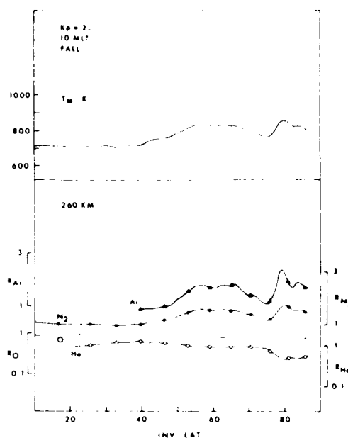
Fig. 2 Latitudinal structure of atmospheric perturbation in the forenoon sector during equinox conditions.
