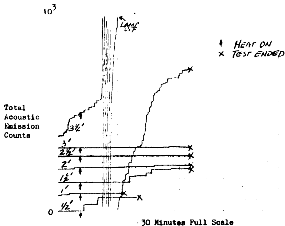
Figure 10. F-111 vertical stabilizer leading edge (A/C 68-005), recorded acoustic emission activity with heating (160° F) at 6" intervals from top of leading edge. 100 db, 175 KHz sensor.
