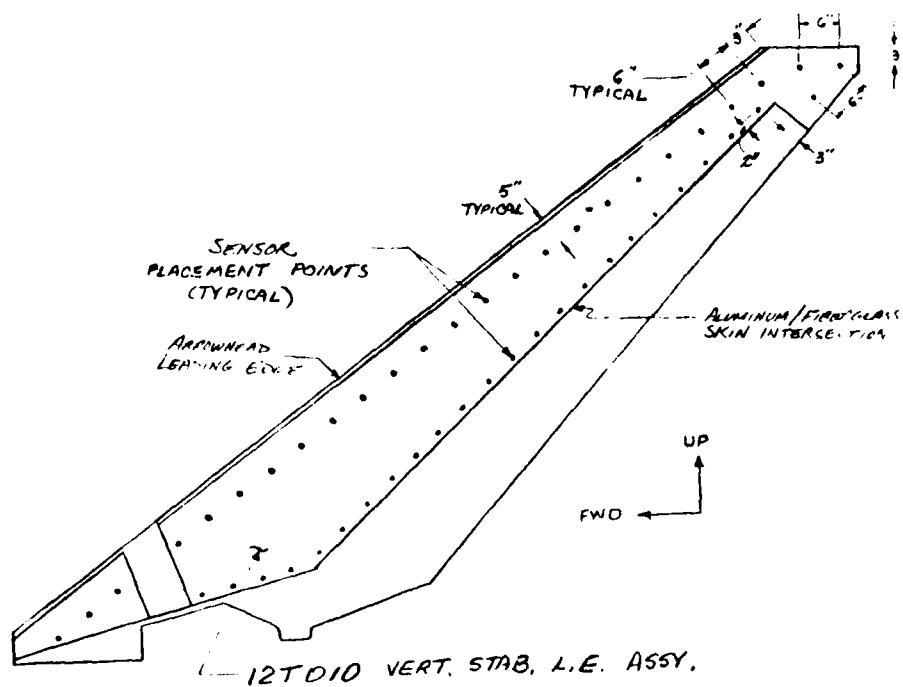
Figure 9. F-111 vertical stabilizer leading edge acoustic emission scanning pattern
