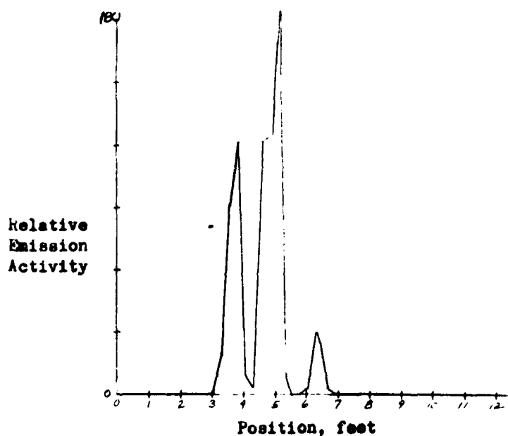
Figure 11. A/C 68-005 vertical leading edge relative acoustic activity with position (see Fig. 10).
