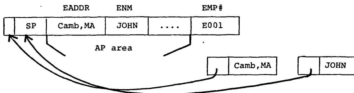
Fig 4.9d: Physical duplication mode; 1:1 Relationship
