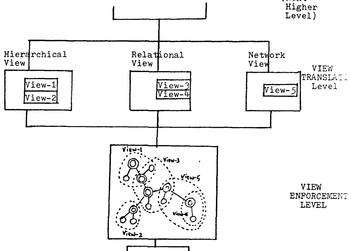
Fig 6.2.1 View Enforcement Level integrates and coordinates views
