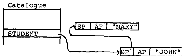
Fig 4.3b: Inserting an element into a primary set
