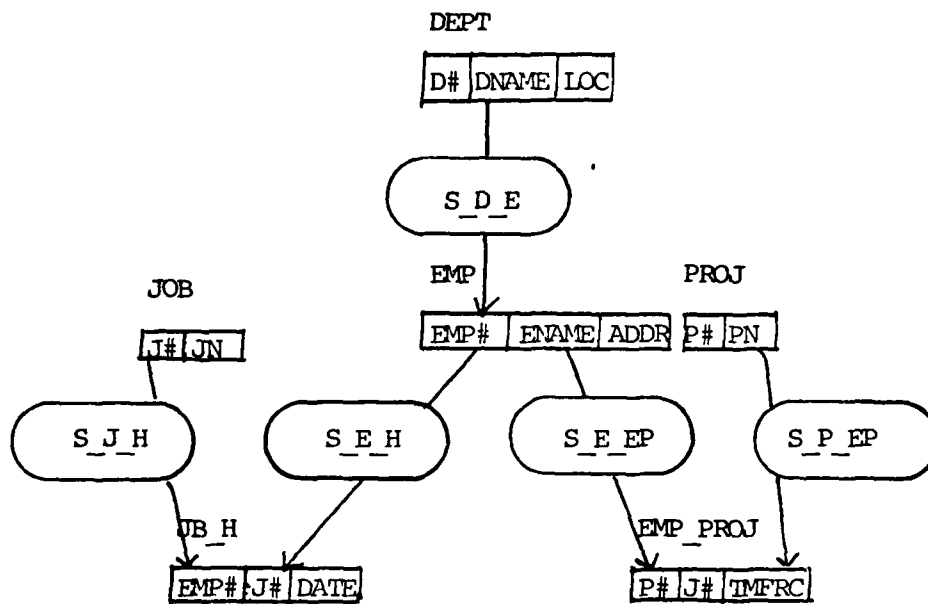
Fig 6.3.9a: A network view of the EMP_ASSIGNMENT database
