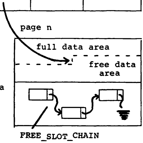
Fig 3.4: Keeping track of available storage space
