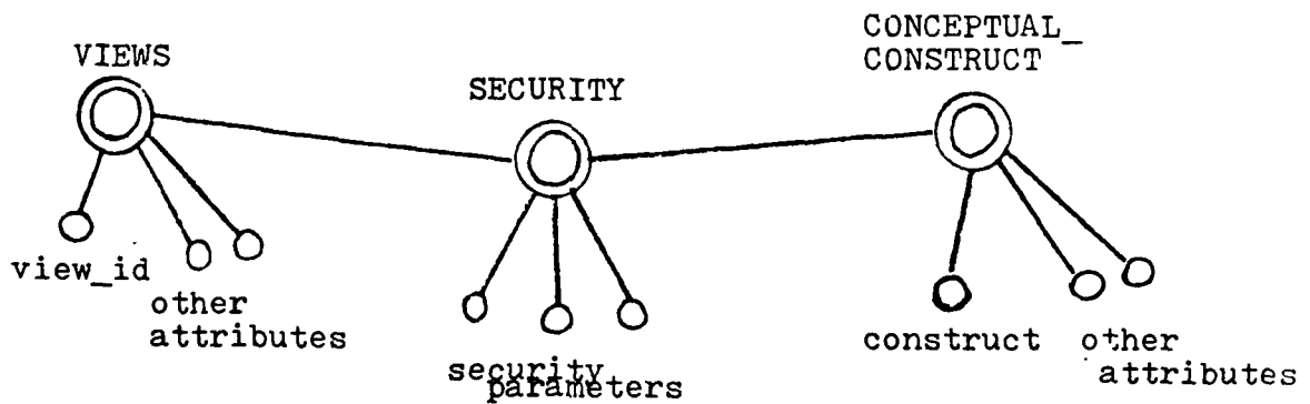
Fig 6.2.2: Catalogue structure at View Enforcement Level
