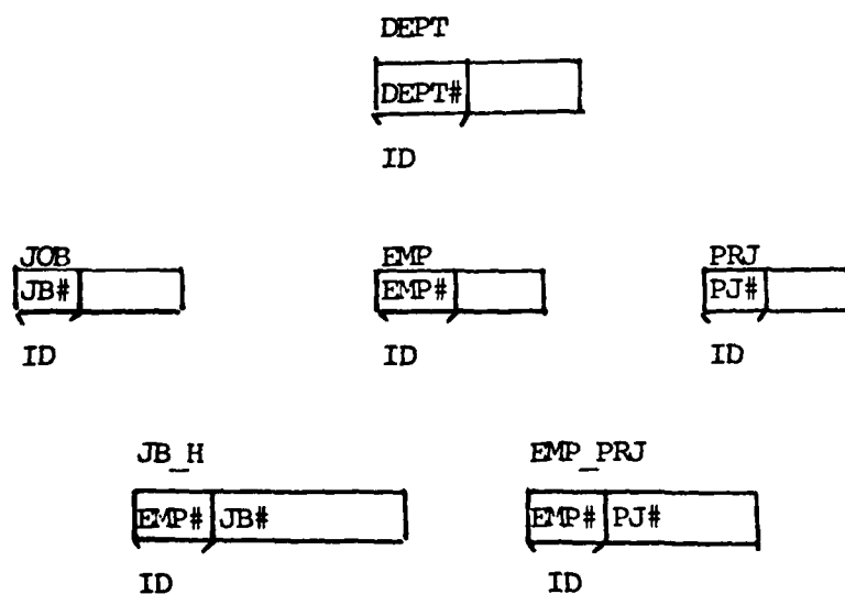
Fig 6.3.11: UWA of EMP_ASSIGNMENT network
