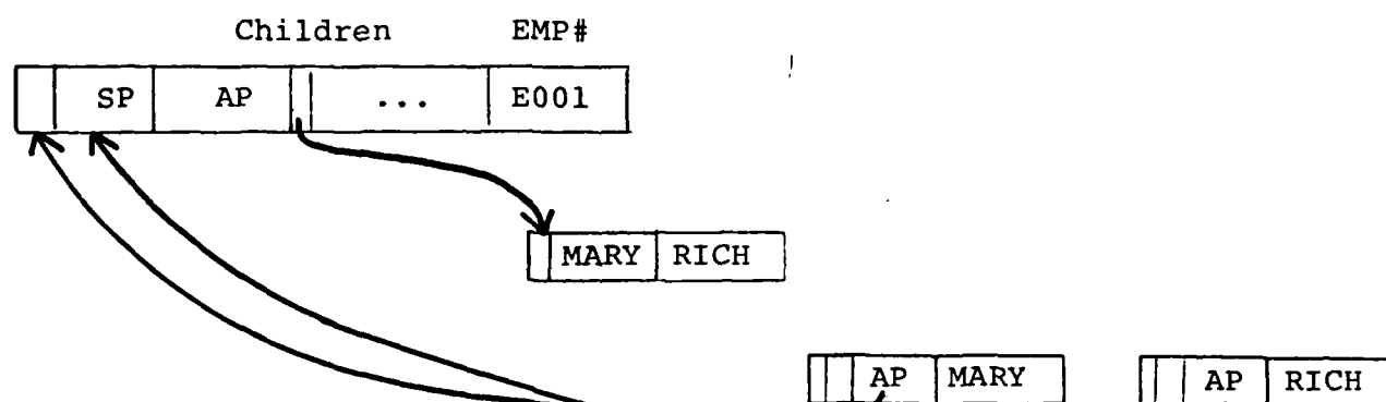
Fig 4.9e: Physical duplication mode; 1:n Relationship
