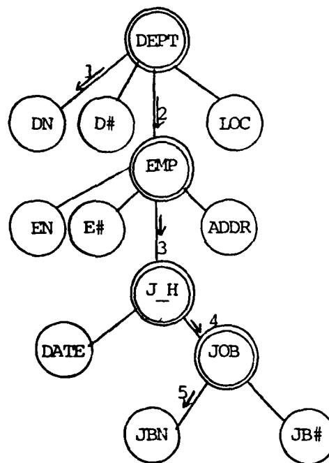
Fig 6.3.8: GU operation: tree form of the retrieval
