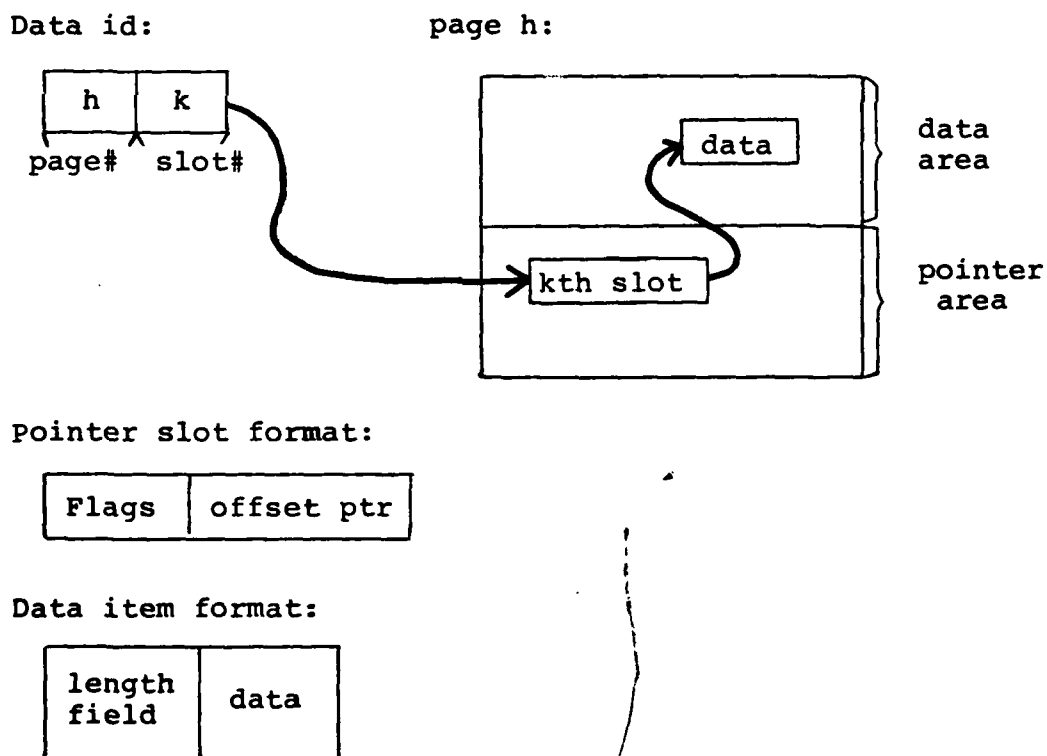
Fig 3.2: The id scheme
