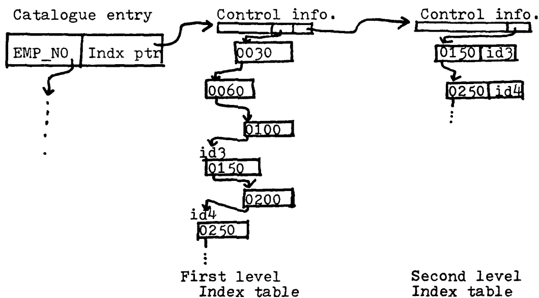
Fig 4.5c: Multi-level index table implementation
