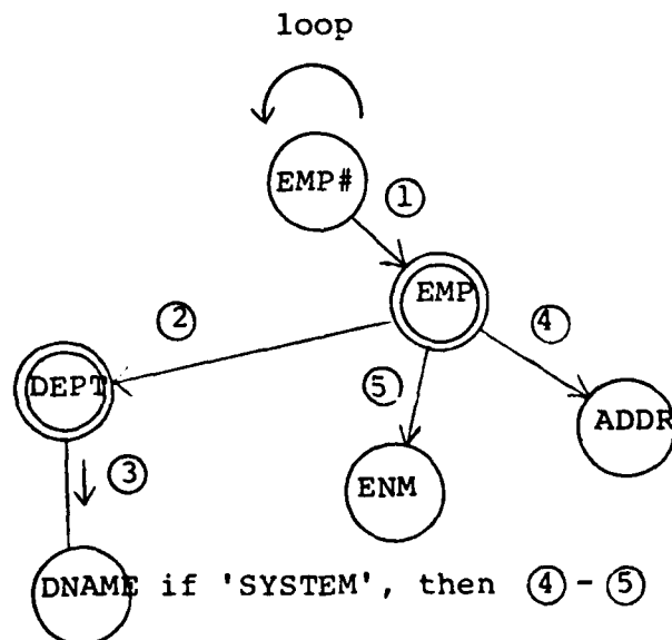
Fig 5.5d: Retrieval strategy 3(b)
