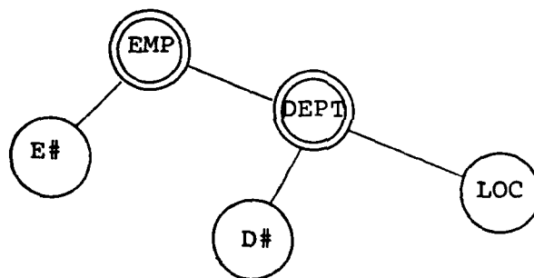
Fig 6.3.3a: Select operation results in a 'pruned' tree
