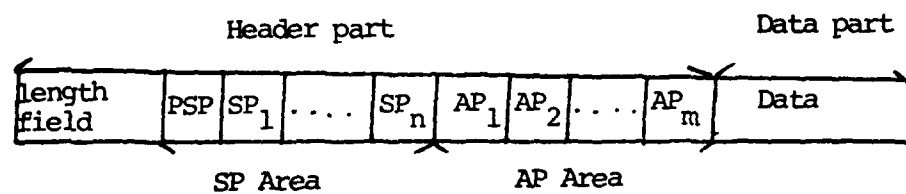
Fig 4.1 Format of a Basic Encoding Unit (BEU)
