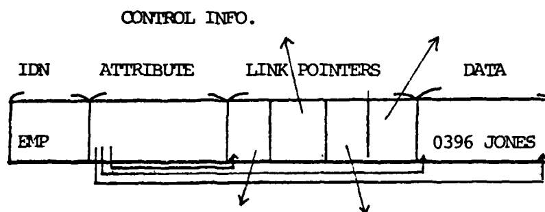
Fig 2.11: Format of a BEU
