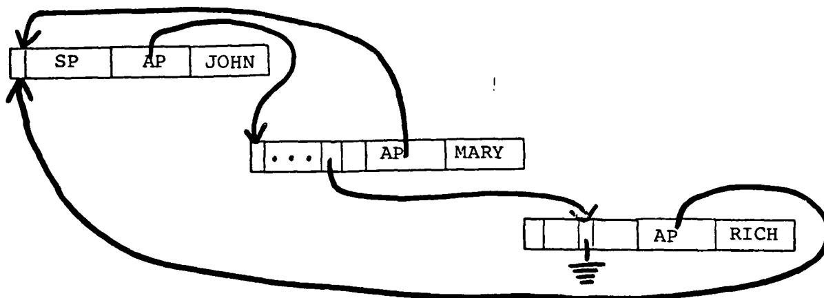
Fig 4.9b: Pointer mode, 1:n (children of JOHN) Relationship
