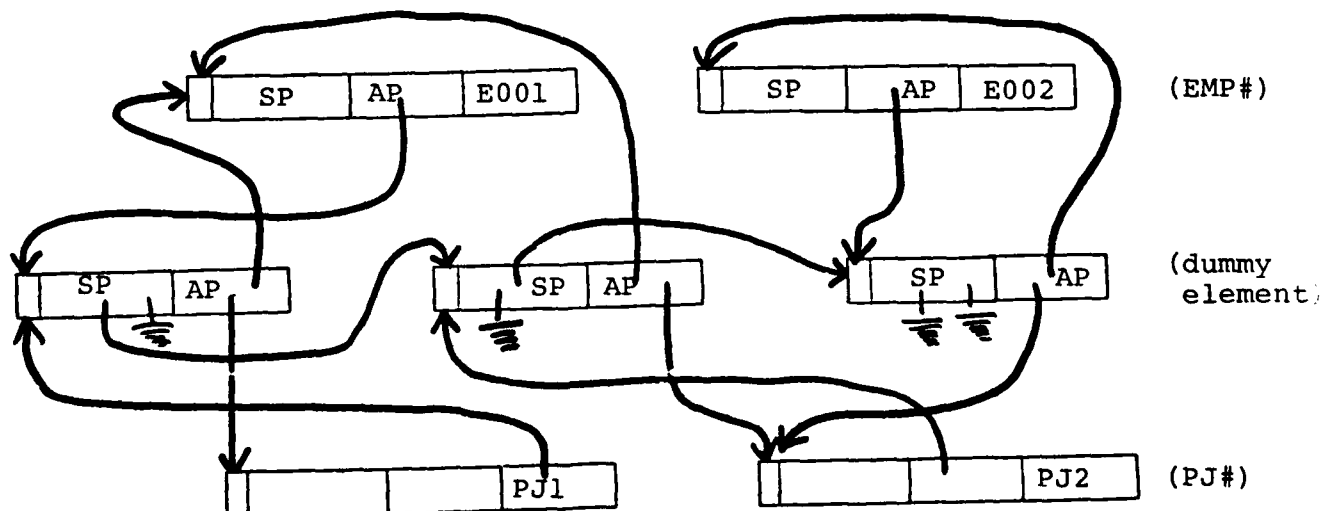
Fig 4.9c: Pointer mode, m:n Relationship (EMP_PROJ)
