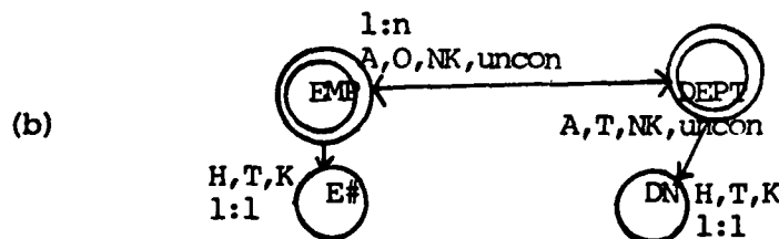
Fig 2.7a & 2.7b: An example schema definition and its BN graph
