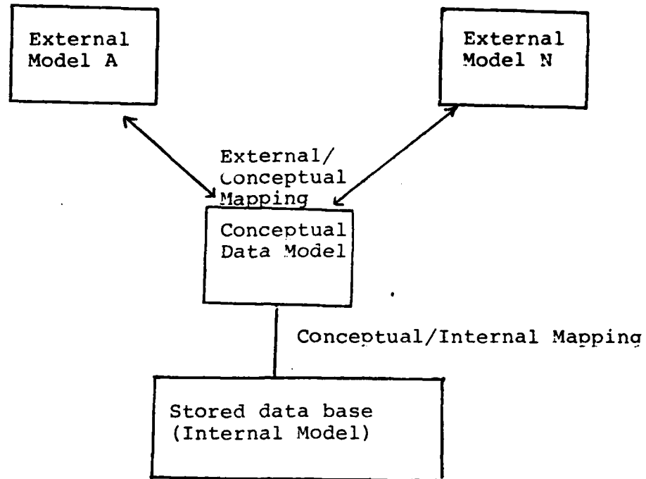
Fig 2.1: The ANSI/SPARC DBMS Architecture
