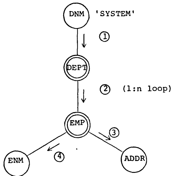
Fig 5.5c: Retrieval strategy 3(a)
