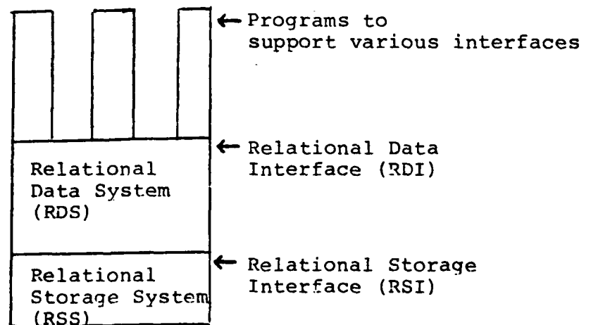
Fig 2.2: The System R Architecture
