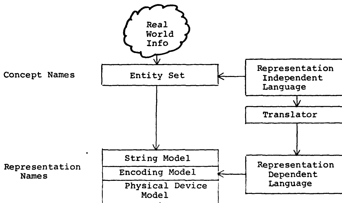
Fig 2.3: The DIAM Architecture
