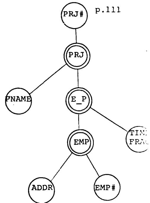
Fig 5.3 & 5.4: Tree forms of access path selection
