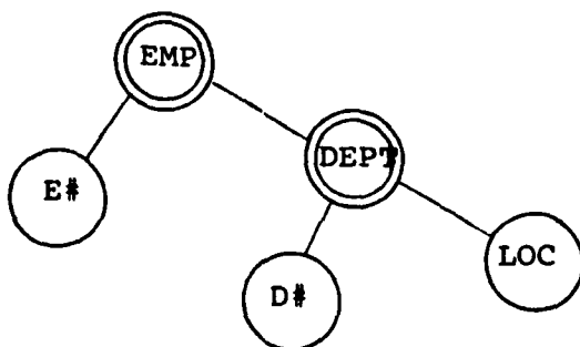
Fig 6.3.3b: D3 is marked not to be output
