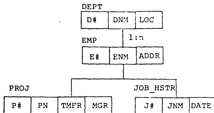
Fig 6.3.5: A Hierarchical view of EMP_ASSIGNMENT
