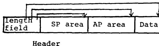
Fig 4.2: Format of an element as it is passed through unary set interface
