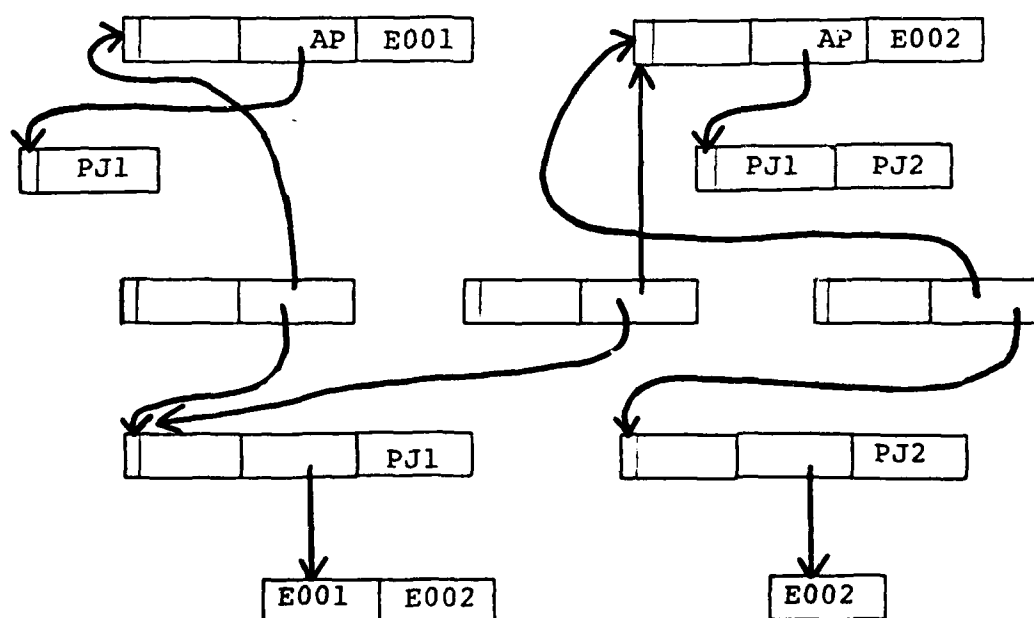
Fig 4.9f: Physical duplication mode; m:n Relationship
