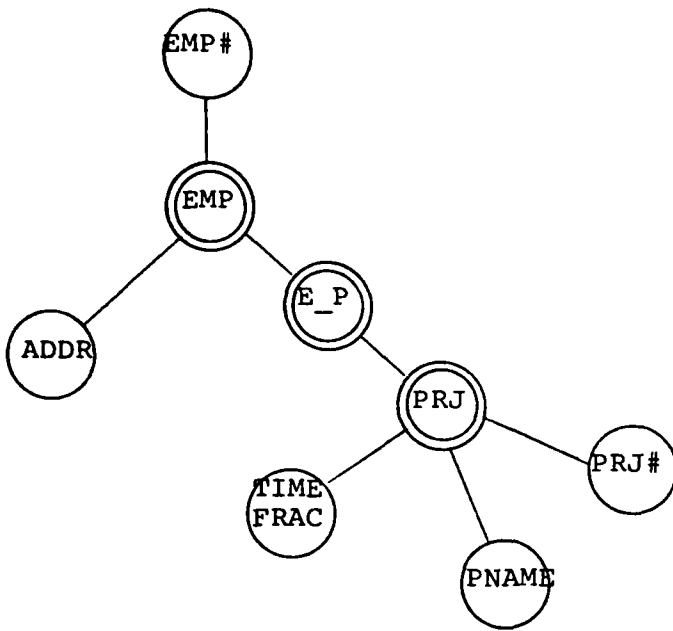
Fig 5.3 & 5.4: Tree forms of access path selection
