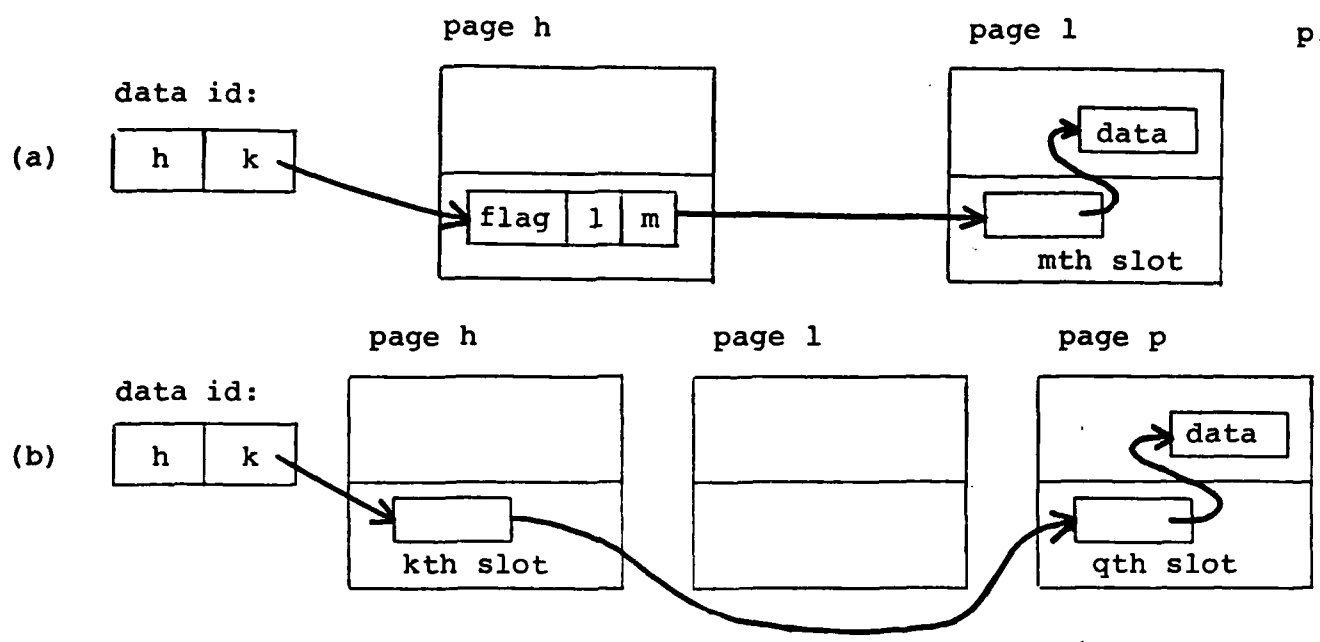
Fig 3.3: Data item moved across pages with id unaffected
