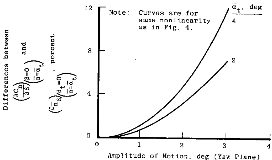
Figure 5. Comparisons of C_{n\beta}^- and \partial C_n^-/\partial\beta values.
