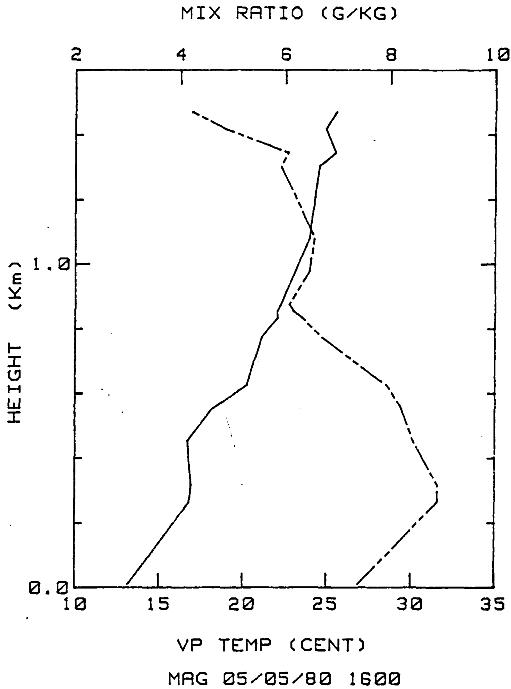
Figure 54. 5 May 1980 at 1600 FD1. ACANIA profile of virtual potential temperature (bottom scale, in degrees Celsius), solid line, and mixing ratio (top scale, in grams per kilogram), broken line, versus height.
