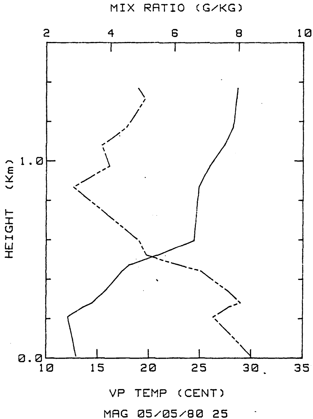
Figure 10. 5 May 1980 at 0025 PDT. ACANZA profile of virtual potential temperature (bottom scale, in degrees Celsius), solid line, and mixing ratio (top scale, in grams per kilogram), dashed line, versus height.
