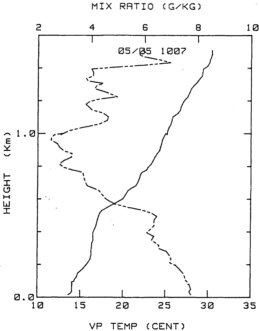
Figure 44. 5 May 1980 at 1007 FDP. Aircraft profile of virtual potential temperature (bottom scale, in degrees Celsius), solid line, and mixing ratio (top scale, in grams per kilogram), broken line, versus height.
