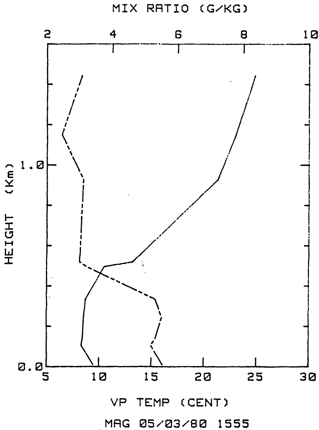
Figure 40. 3 May 1980 at 1555 EDT. ACANIA profile of virtual potential temperature (bottom scale, in degrees Celsius), solid line, and mixing ratio (top scale, in grams per kilogram), broken line, versus height.
