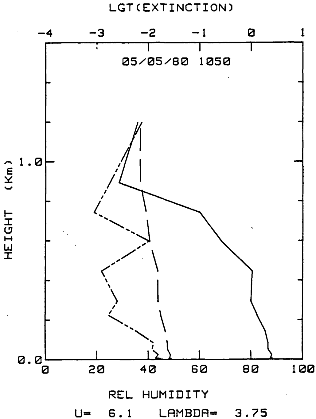
Figure 55. 5 May 1980 at 1050 FDL profile of relative humidity (bottom scale) solid line, observed extinction coefficients (top scale), series of short solid and dashed lines, and predicted extinction coefficients, series of short solid lines versus height. Top scale is logarithmic, where 1 is 10. Wind speed at 6.1 m/s and wavelength (LAMBDA) at 3.75 microns.
