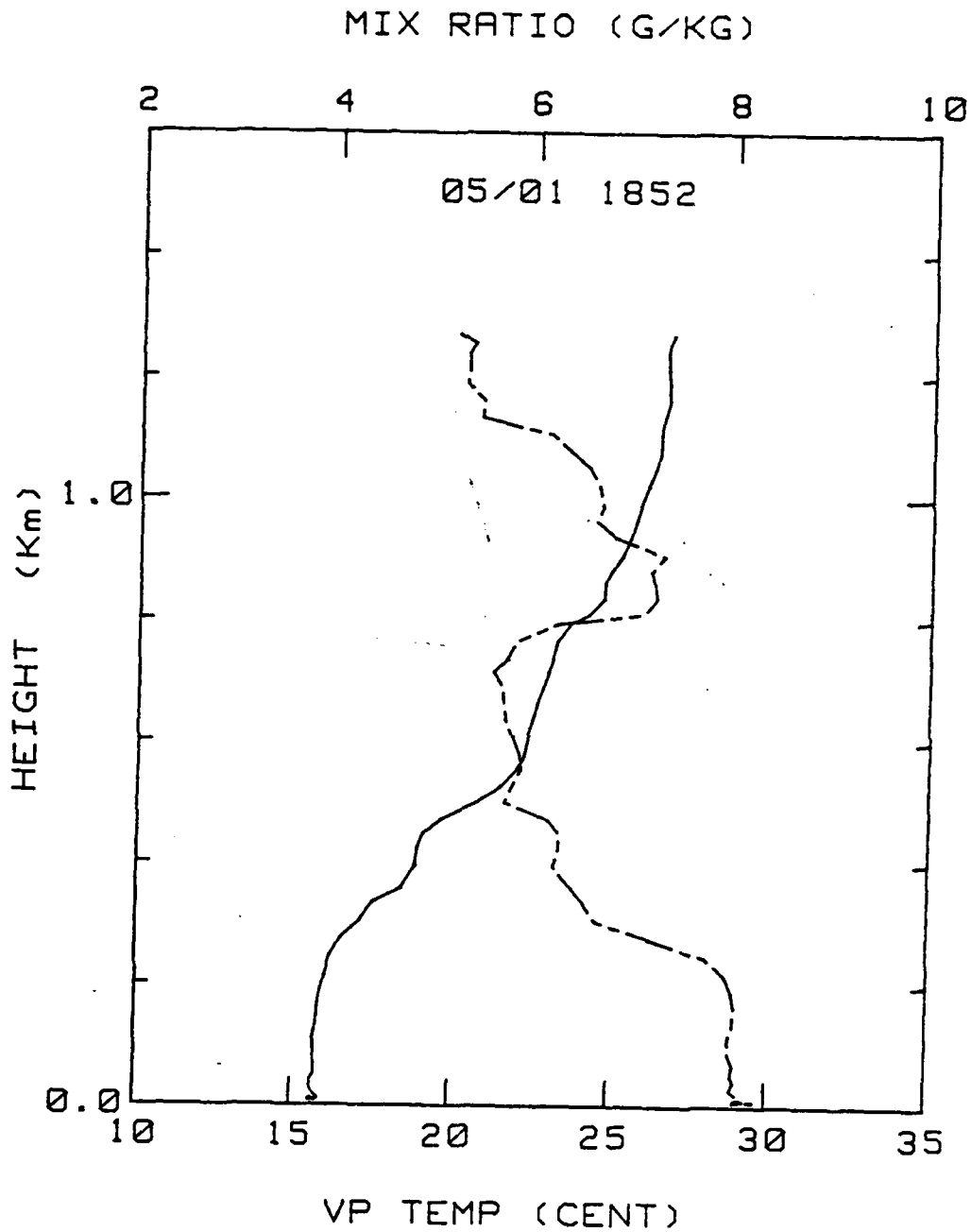
Figure 28. 1 May 1980 at 1852 EDT. Aircraft profile of virtual potential temperature (bottom scale, in degrees Celsius), solid line, and mixing ratio (top scale, in grams per kilogram), broken line, versus height.
