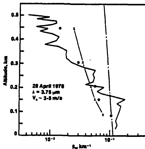
(a) Aerosol extinction coefficient variation with altitude calculated using aerosol size distributions measured during constant altitude (●) and spiral (—) aircraft flights; the WGM model (X—X); and the LOWTRAN 3B maritime model (---).
