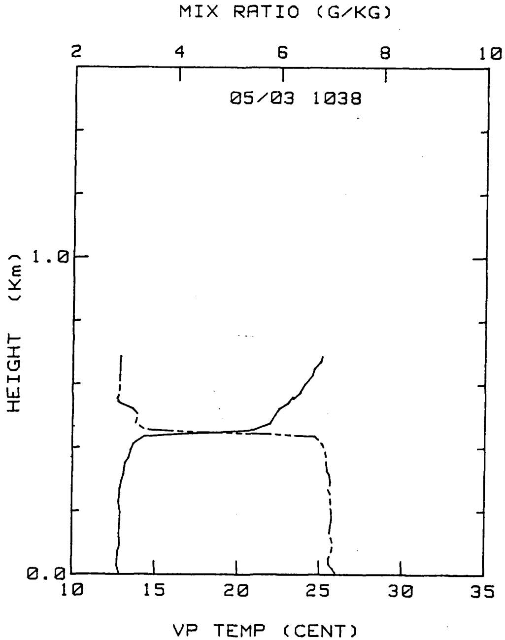
Figure 33. 3 May 1980 at 1038 PDT. Aircraft profile of virtual potential temperature (bottom scale, in degrees Celsius), solid line, and mixing ratio (top scale, in grams per kilogram), broken line, versus height.
