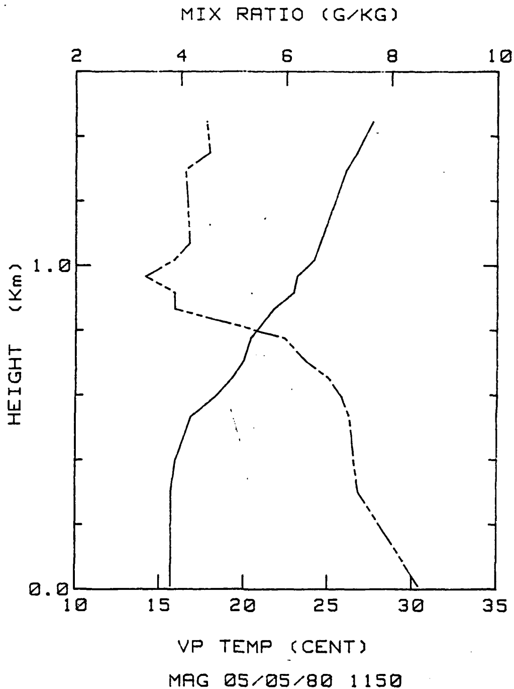
Figure 52. 5 May 1980 1150 PDT. NCAR profile of virtual potential temperature (bottom scale, in degrees Celsius), solid line, and mixing ratio (top scale, in grams per kilogram), broken line, versus height.
