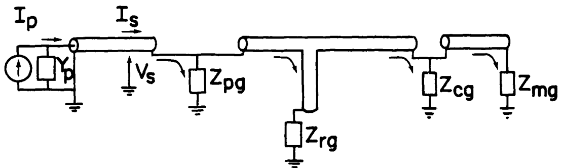
Figure 10. Propagation of Penetrating Power Current to Internal Circuits (a) Internal Propagation -- Conductor/Shield Mode (b) Shield Excitation by Internal Voltage and Current
