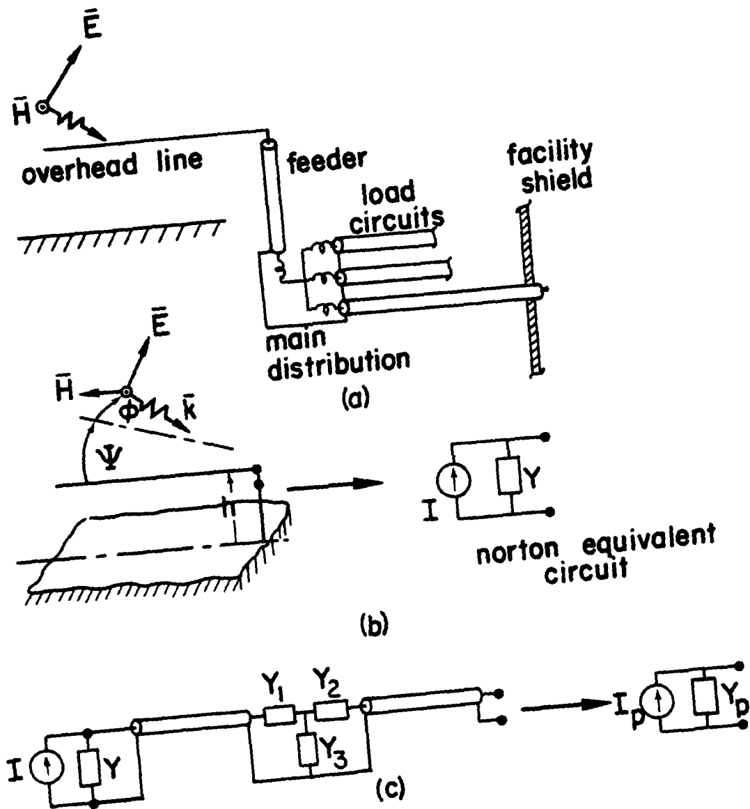
Figure 4. External Coupling and Propagation Through AC Power System (a) AC Power Circuits (b) Equivalent Source for Overhead Lines (c) Source Transferred to Facility Shield Penetration
