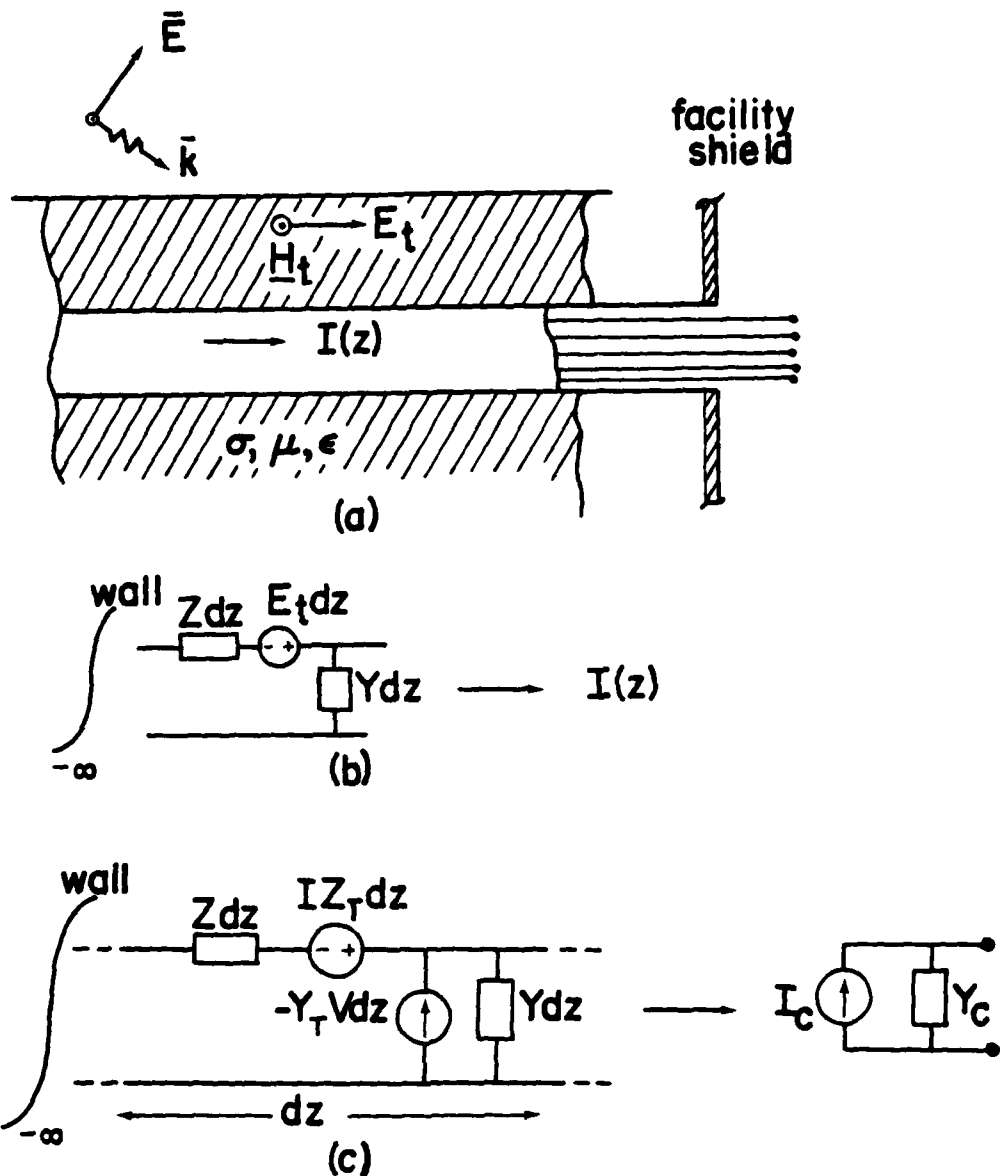
Figure 5. External Coupling and Propagation Through Shielded Underground Communication Cable
