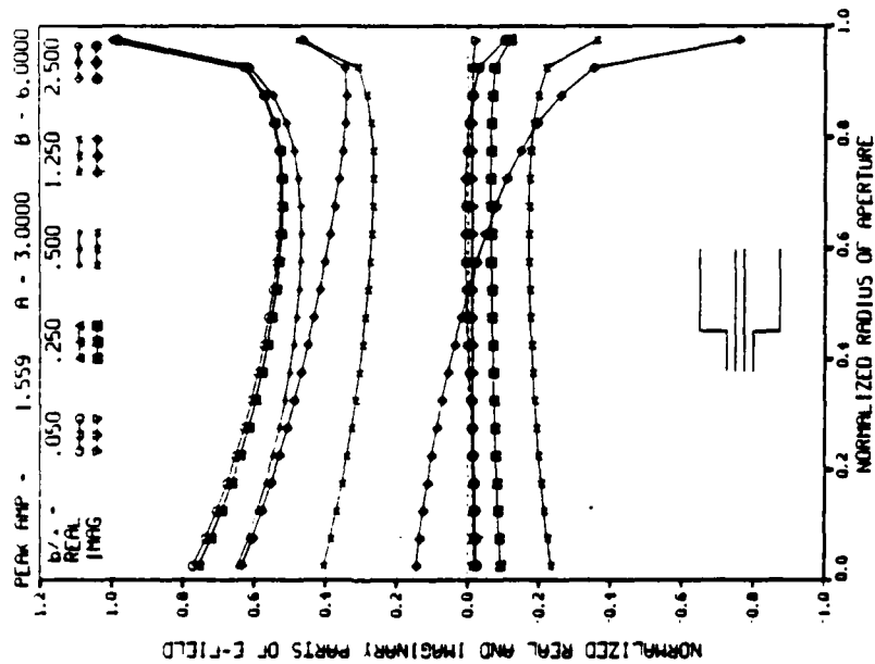
FIGURE 10 CALCULATED DISTRIBUTIONS OF APERTURE ELECTRIC FIELD FOR STEP IN OUTER RADIUS
