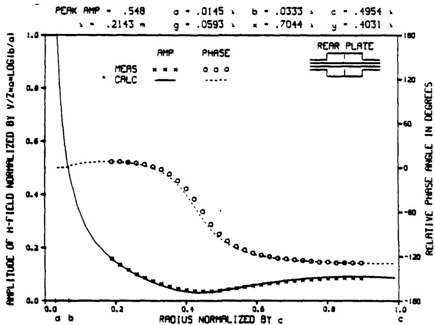
FIGURE 66 MEASURED AND CALCULATED \theta COMPONENT OF MAGNETIC FIELD 1400 MHZ
