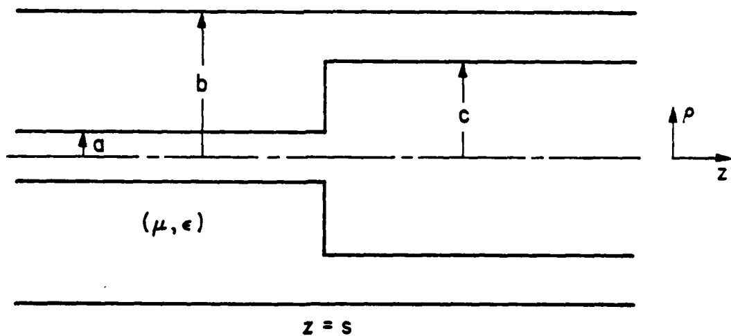
Figure 4b. Step Discontinuity in the Inner Conductor of a Coaxial Waveguide
