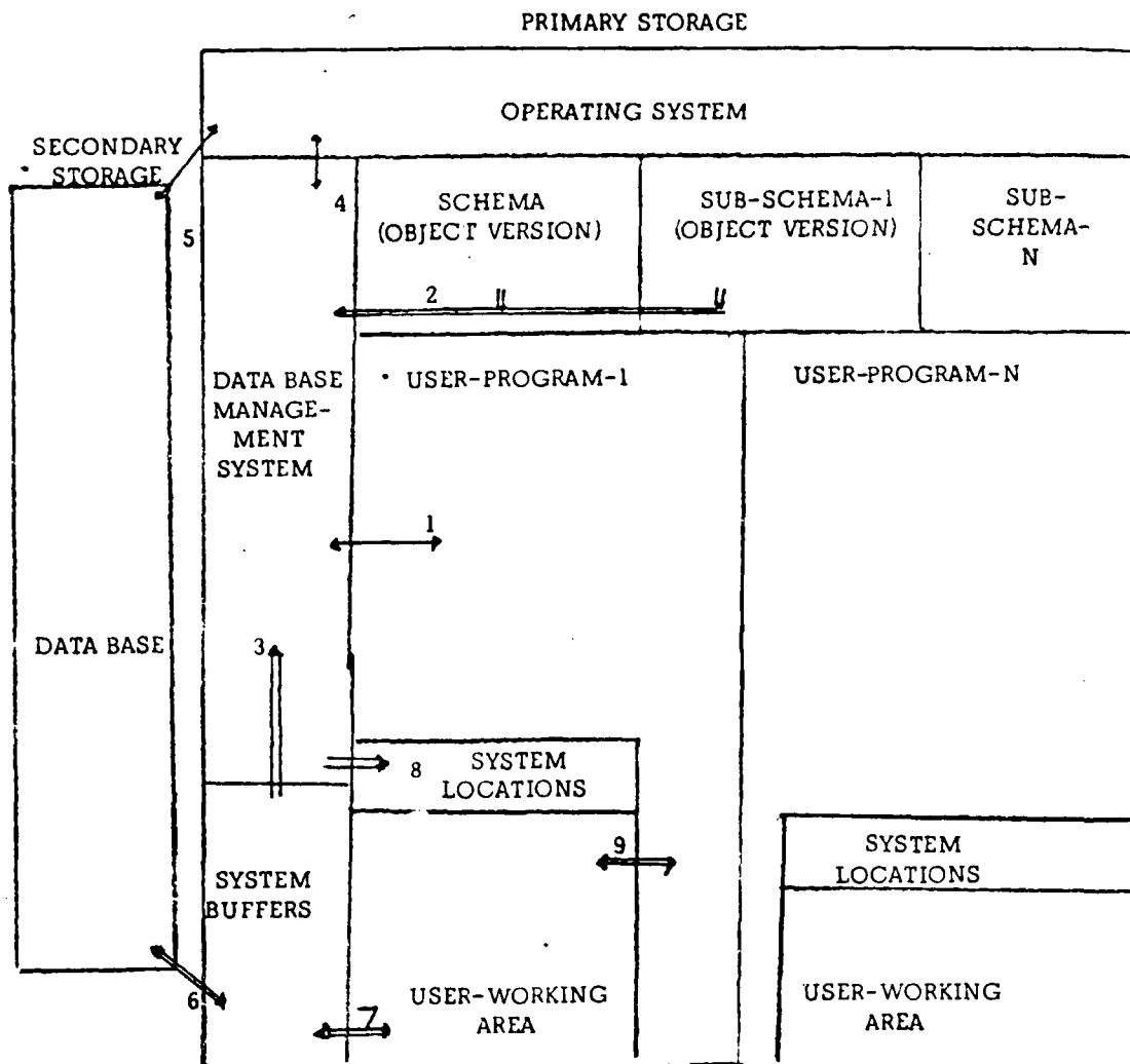
Figure 3 DBMS Memory Layout and Operation
