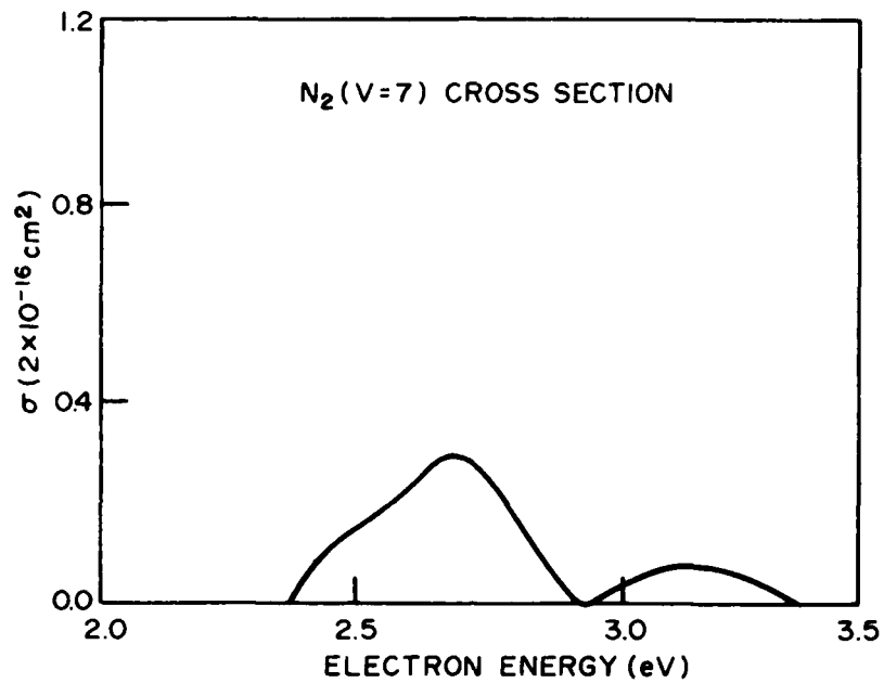
Fig. 7 — The cross section for the electron impact excitation of the seventh ground state vibrational level of \text{N}_2
