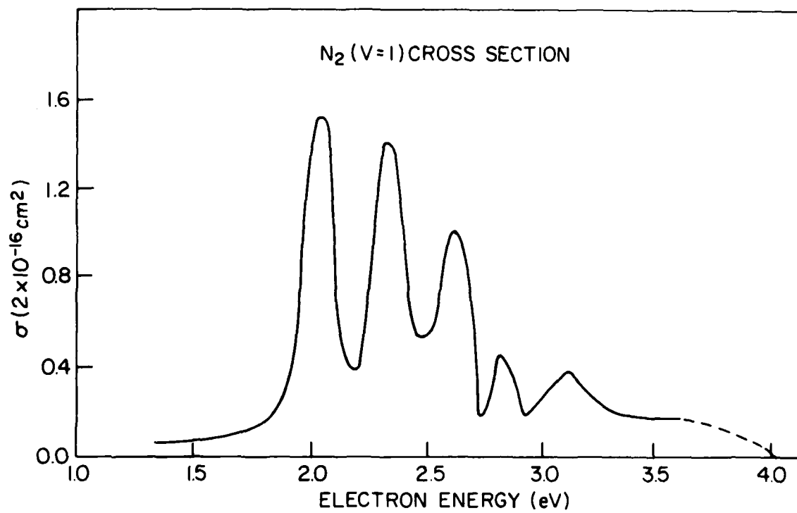
Fig. 1 — The cross section for the electron impact excitation of the first ground state vibrational level of \text{N}_2
