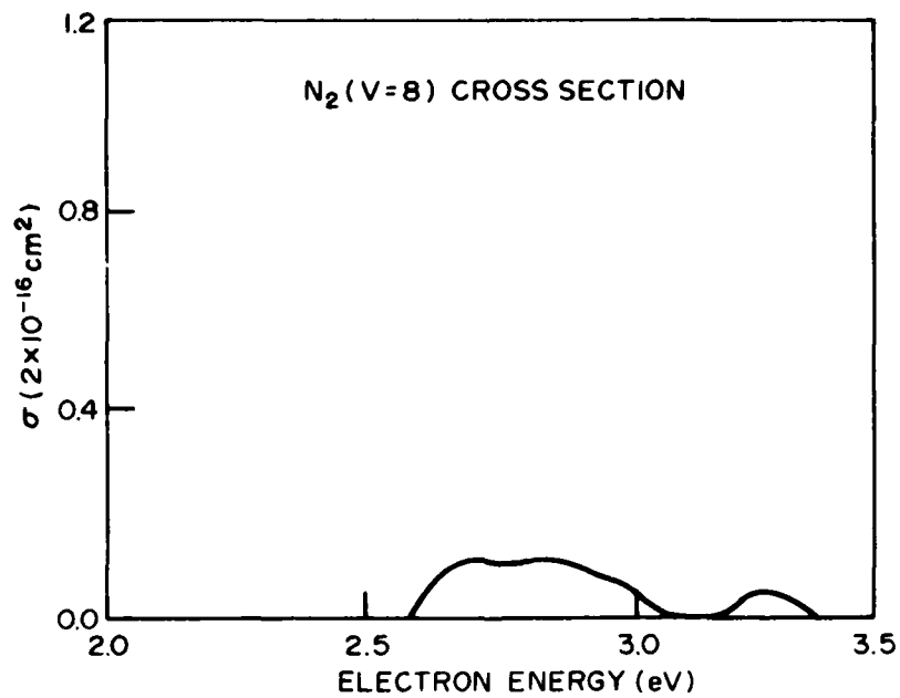
Fig. 8 — The cross section for the electron impact excitation of the eighth ground state vibrational level of \text{N}_2
