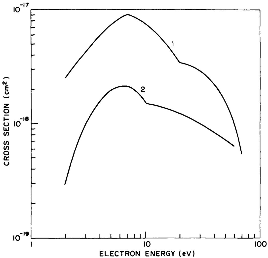
Fig. 24 — The electron impact excitation cross section of O 2 (a 1 Δ) and b 1 Σ. (See text for references.)
