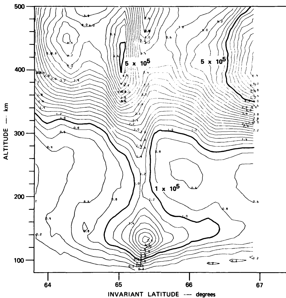
FIGURE 12 ALTITUDE/LATITUDE VARIATION OF ELECTRON DENSITY — 23 FEBRUARY 1980, 114043 TO 115316 UT
